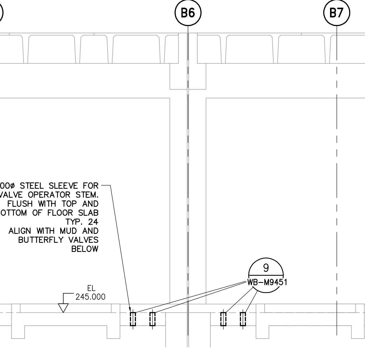
P SECTION - FLOOR SLEEVE INSTALLATION FOR VALVE OPERATOR STEMS - TYP. 24 WP-M9103 1:50
