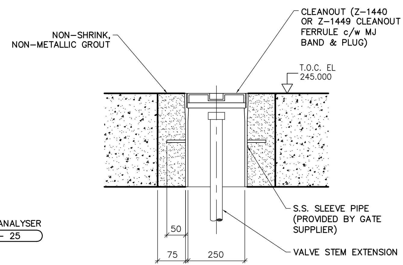
1 DETAIL - CAST IN PLACE FLOOR BOX WP-M9105 NTS WP-M9103
