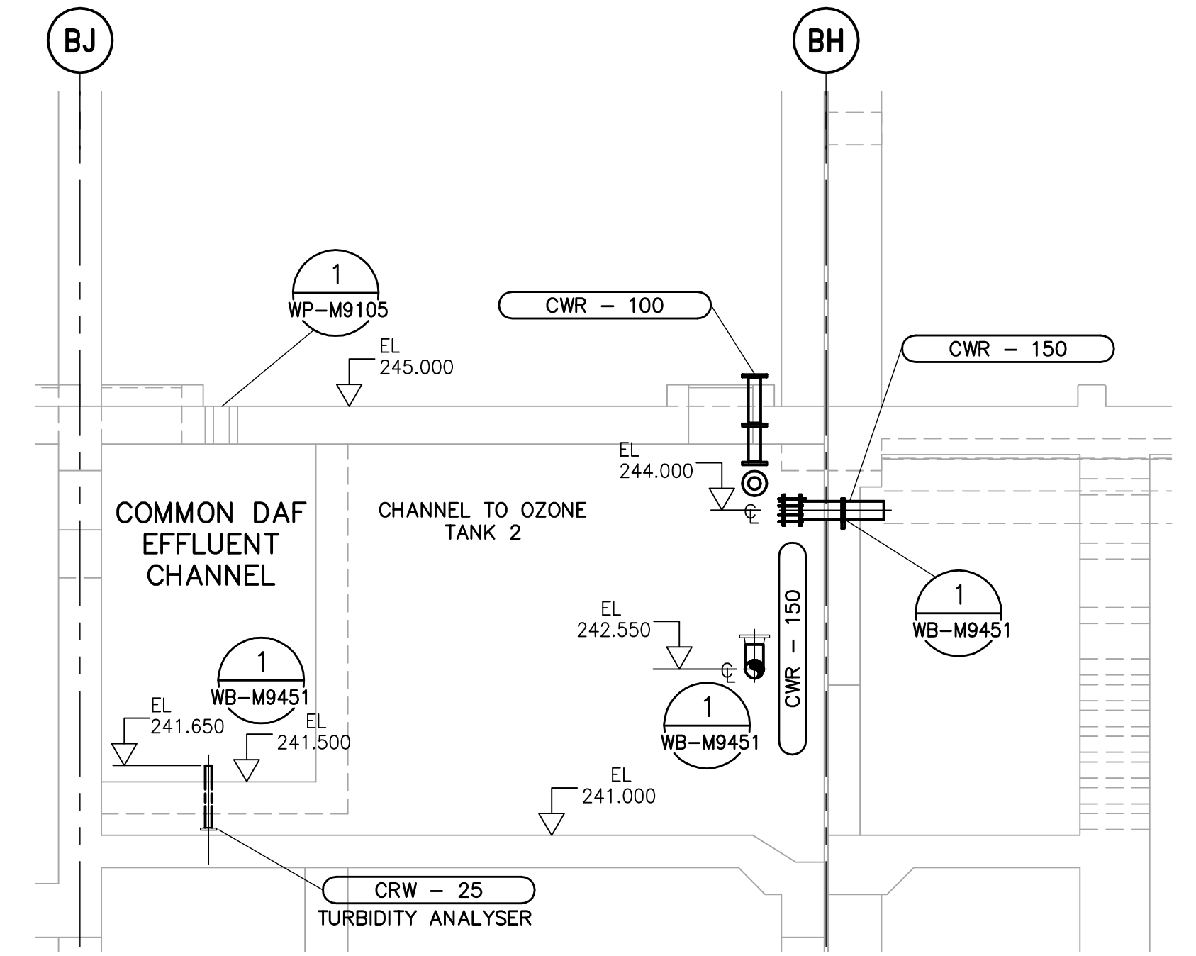
N SECTION - OZONE COOLING WATER RETURN WP-M9105 1:50
