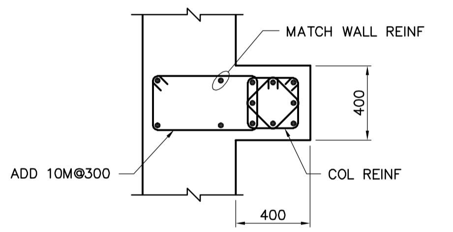
1 - 1:20 DETAIL
