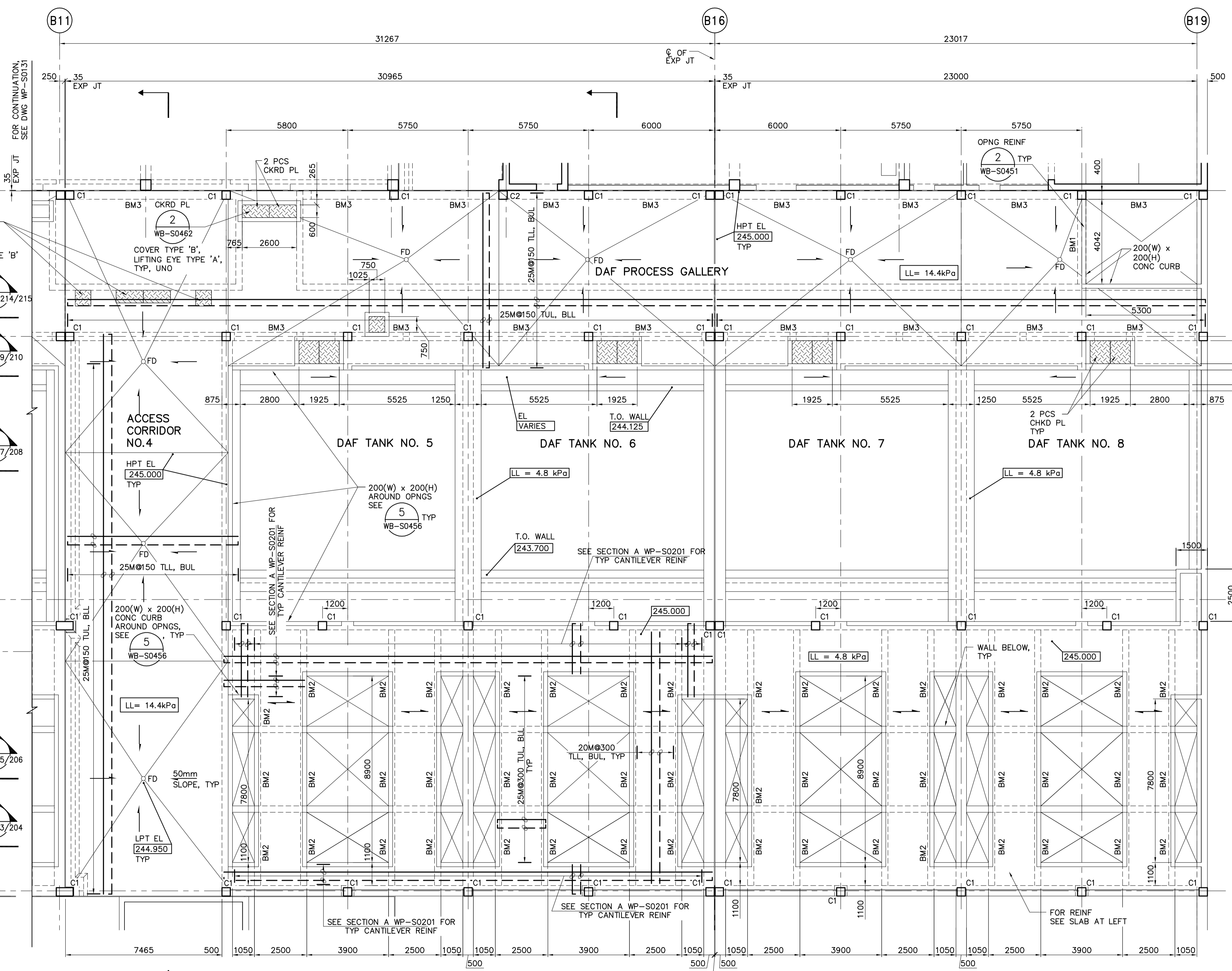
THIRD FLOOR PLAN 1:100
