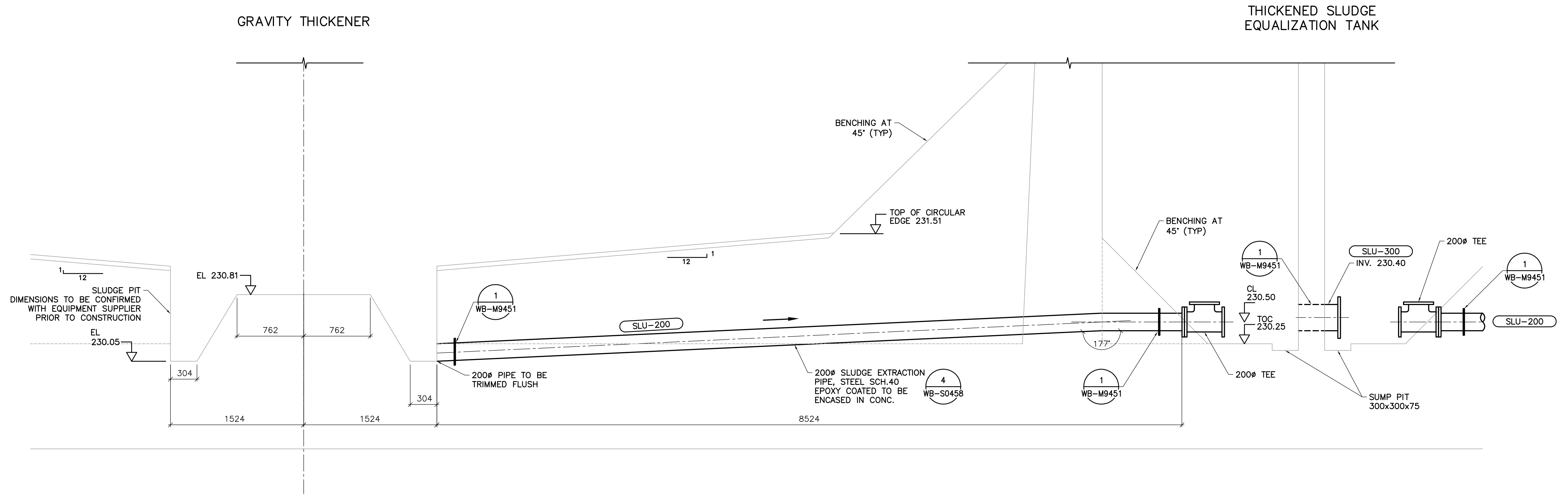
F SECTION WR-M9123 1:25
