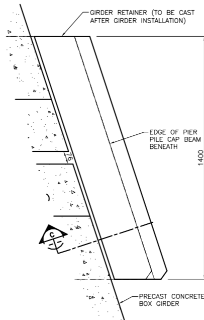
GIRDER RETAINER DETAIL 1:10
