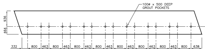
GROUT POCKET LOCATION DETAIL 1:50
