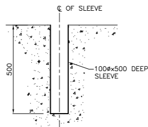
GROUT POCKET DETAIL 1:10
