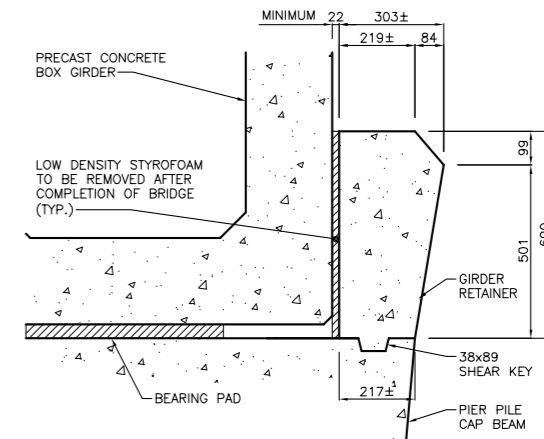
GIRDER RETAINER SECTION C 1:16
