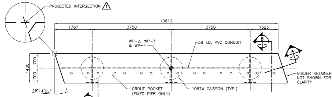
PIER PLAN 1:50
