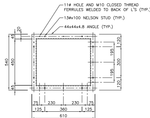
LIGHT FIXTURE ANCHOR DETAIL 1:10
