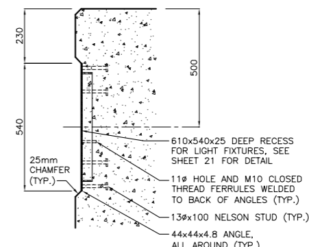
LIGHT FIXTURE RECESS DETAIL 1:25
