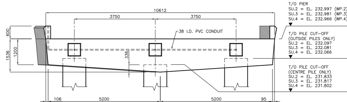
PIER SECTION A 1:50
