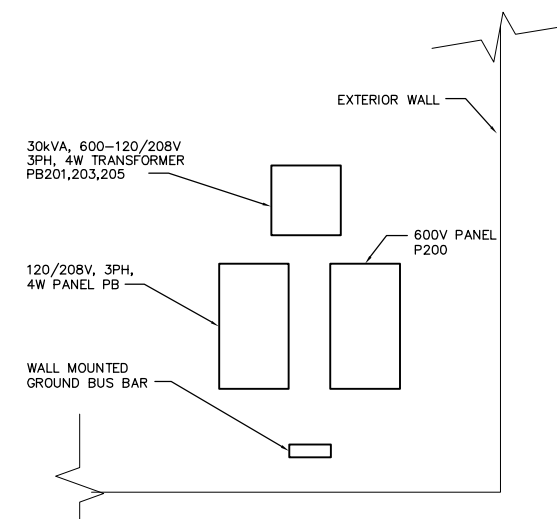
1 DISTRIBUTION EQUIPMENT MOUNTING DETAIL SCALE: N.T.S.
