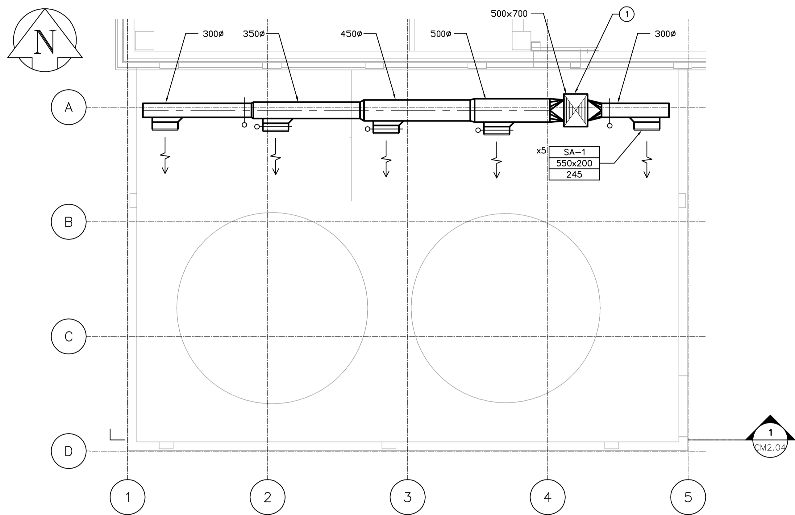
HVAC PLAN - MAIN LEVEL SCALE: 1:50
