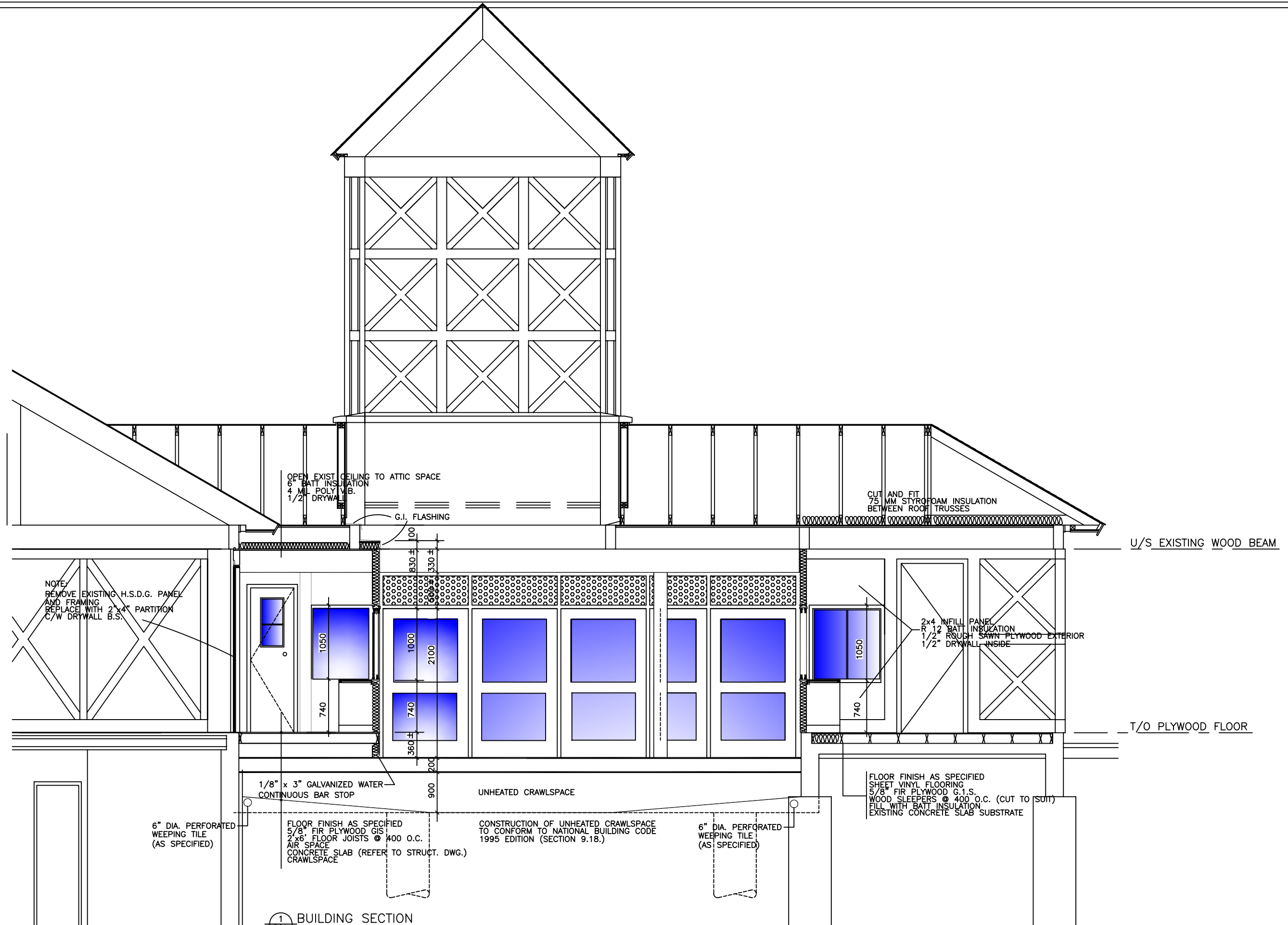
1 BUILDING SECTION 2/4 SCALE 1:50
