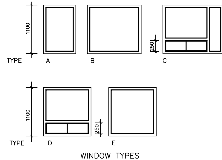
WINDOW TYPES
