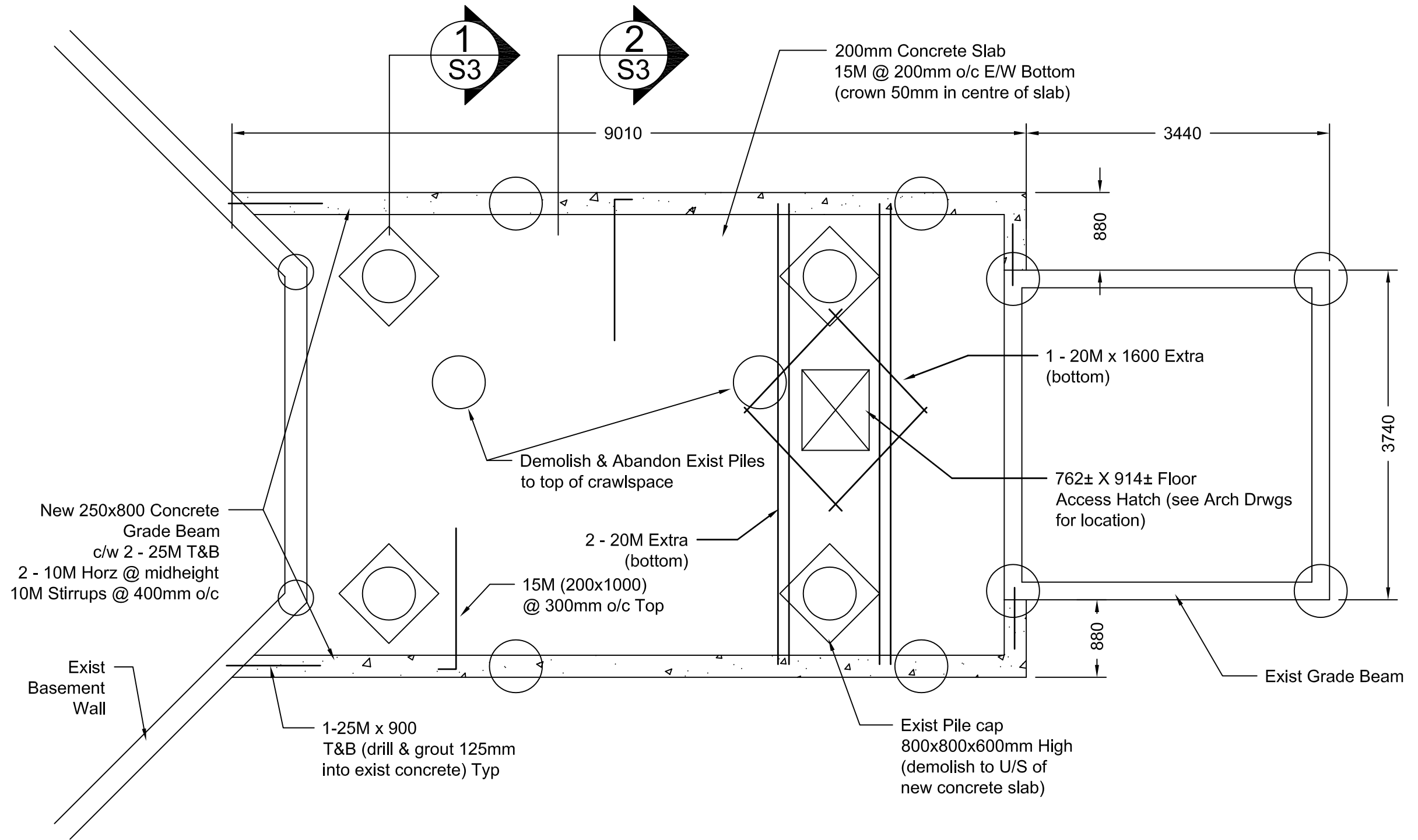
MAIN FLOOR PLAN SCALE 1:50
