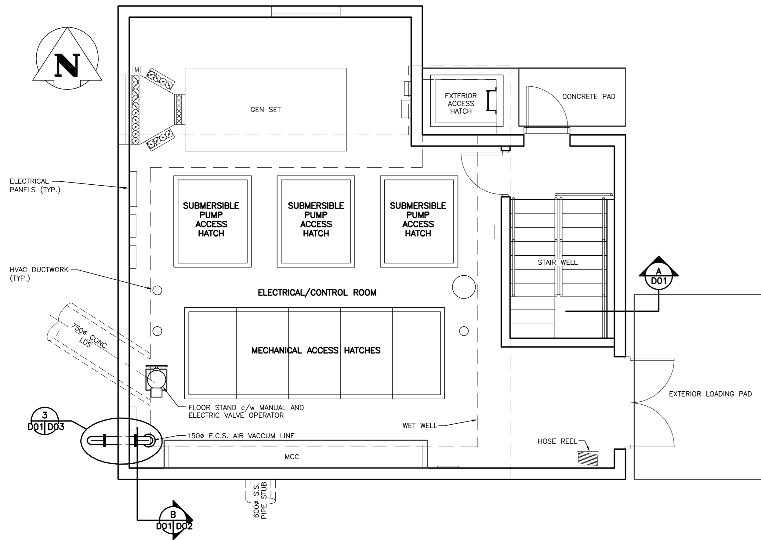
MAIN FLOOR PLAN 1:50
