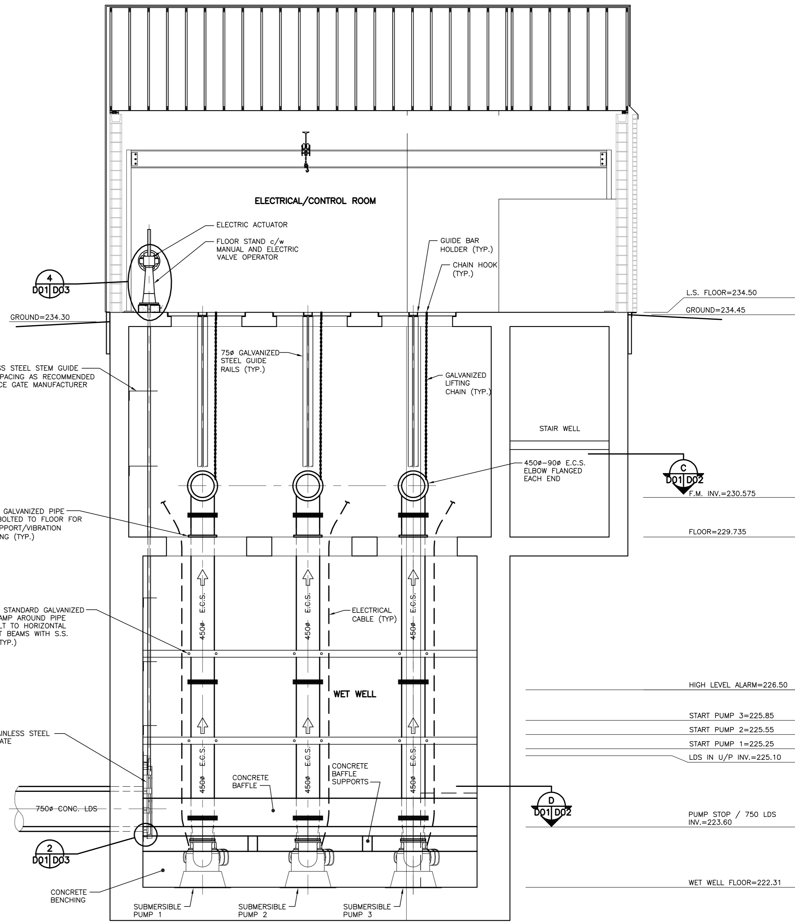
SECTION D01 1:50
