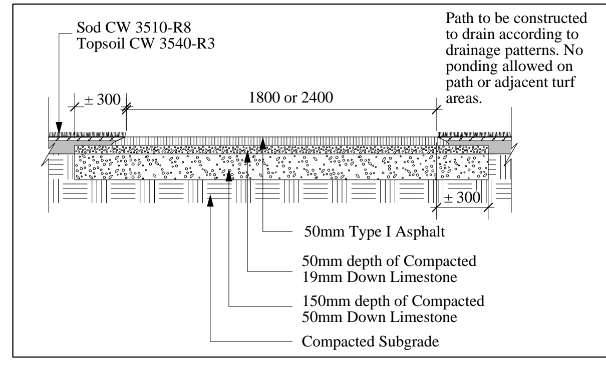
3 L2 Asphalt Path Section 1:25
