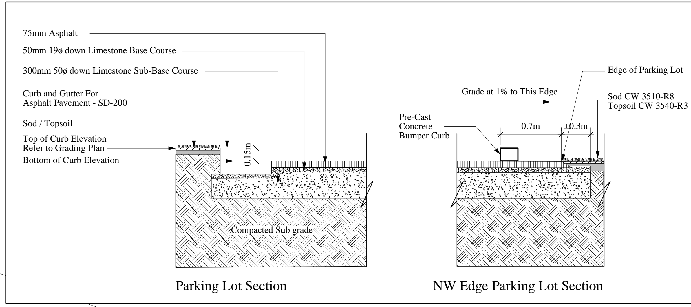
2 L2 Parking Lot Sections 1:25
