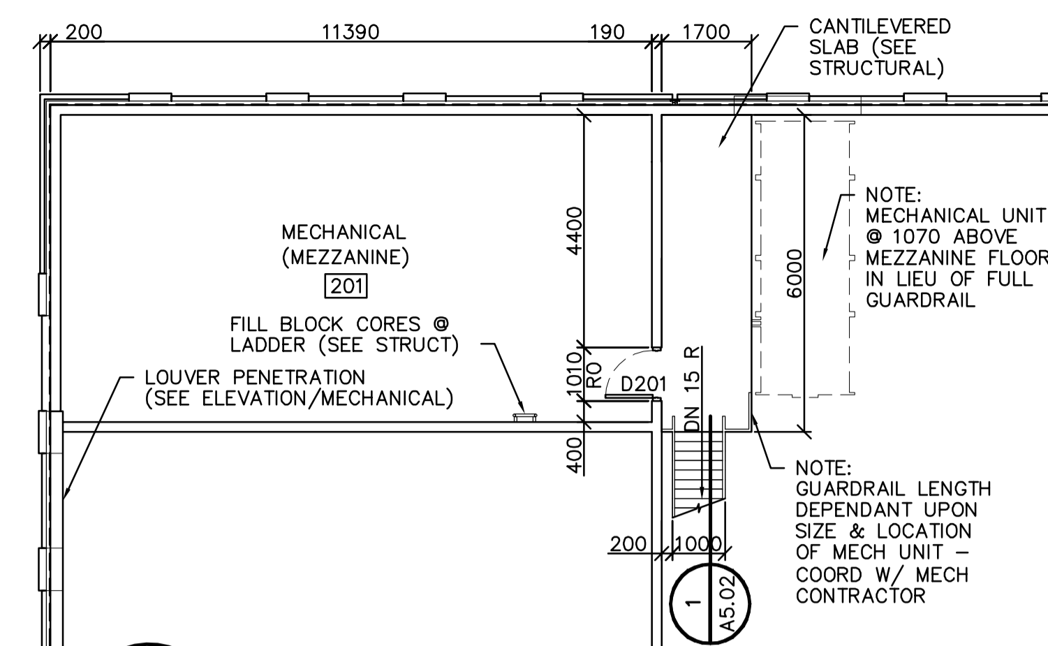
MEZZANINE FLOOR PLAN SCALE 1:100
