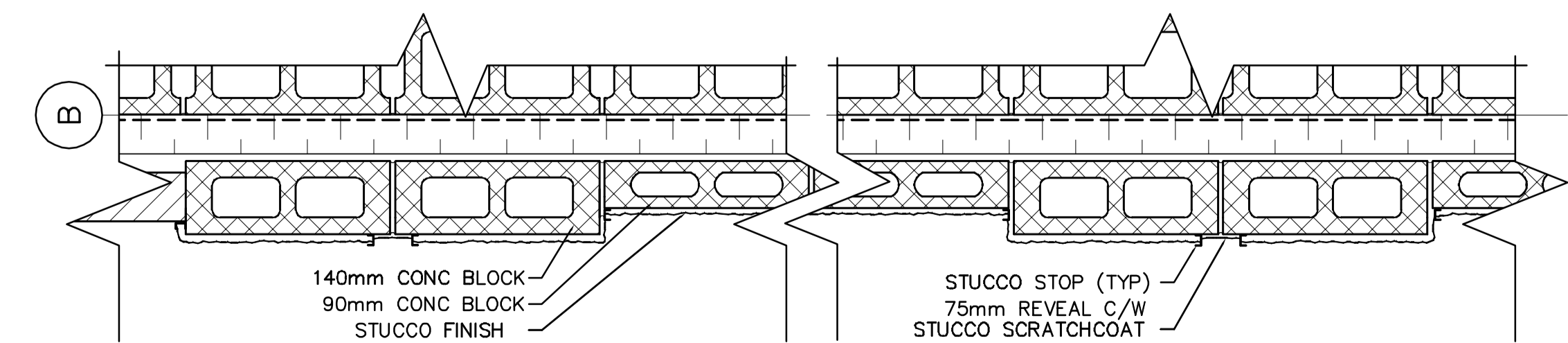
3 TYPICAL PLAN DETAIL @ STUCCO REVEAL SCALE 1:10
