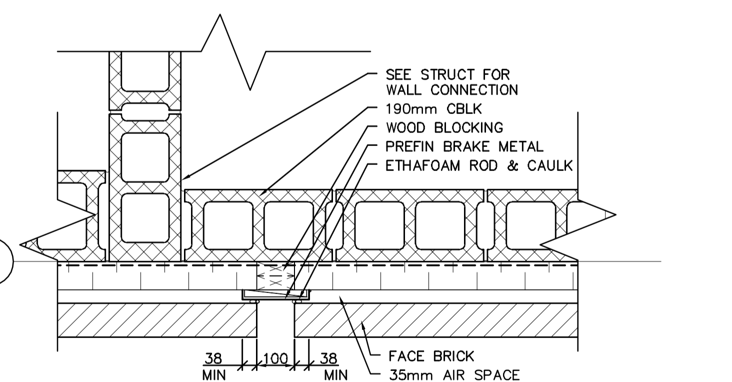
2 PLAN DETAIL @ REVEAL/CONTROL JOINT SCALE 1:10
