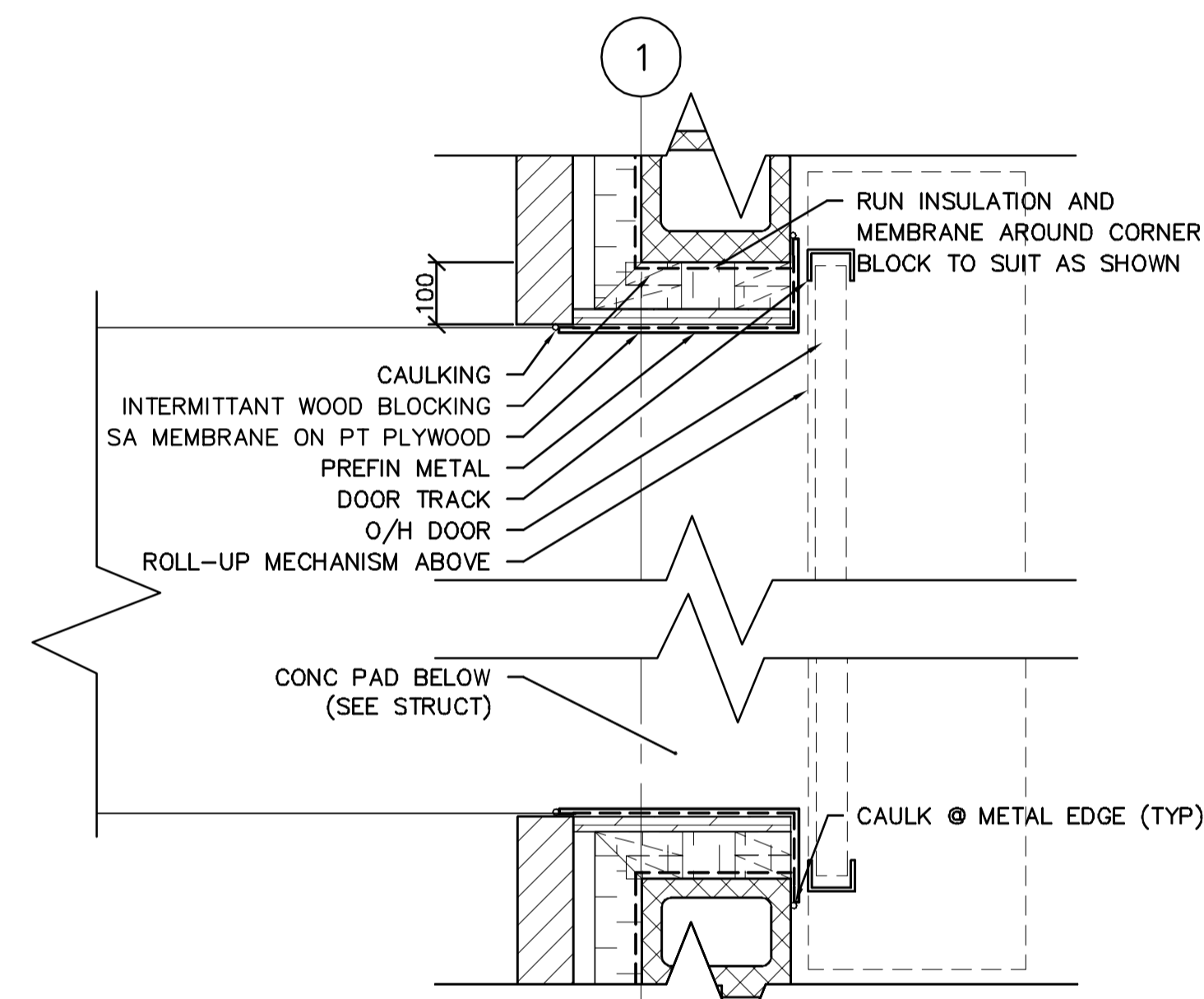
1 PLAN DETAIL @ LOADING DOOR SCALE 1:10
