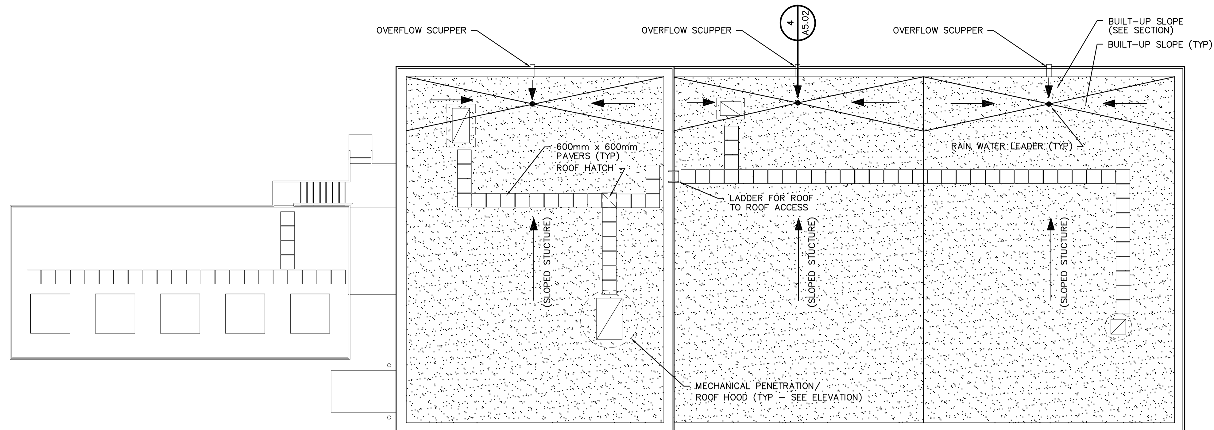
ROOF PLAN SCALE 1:100
