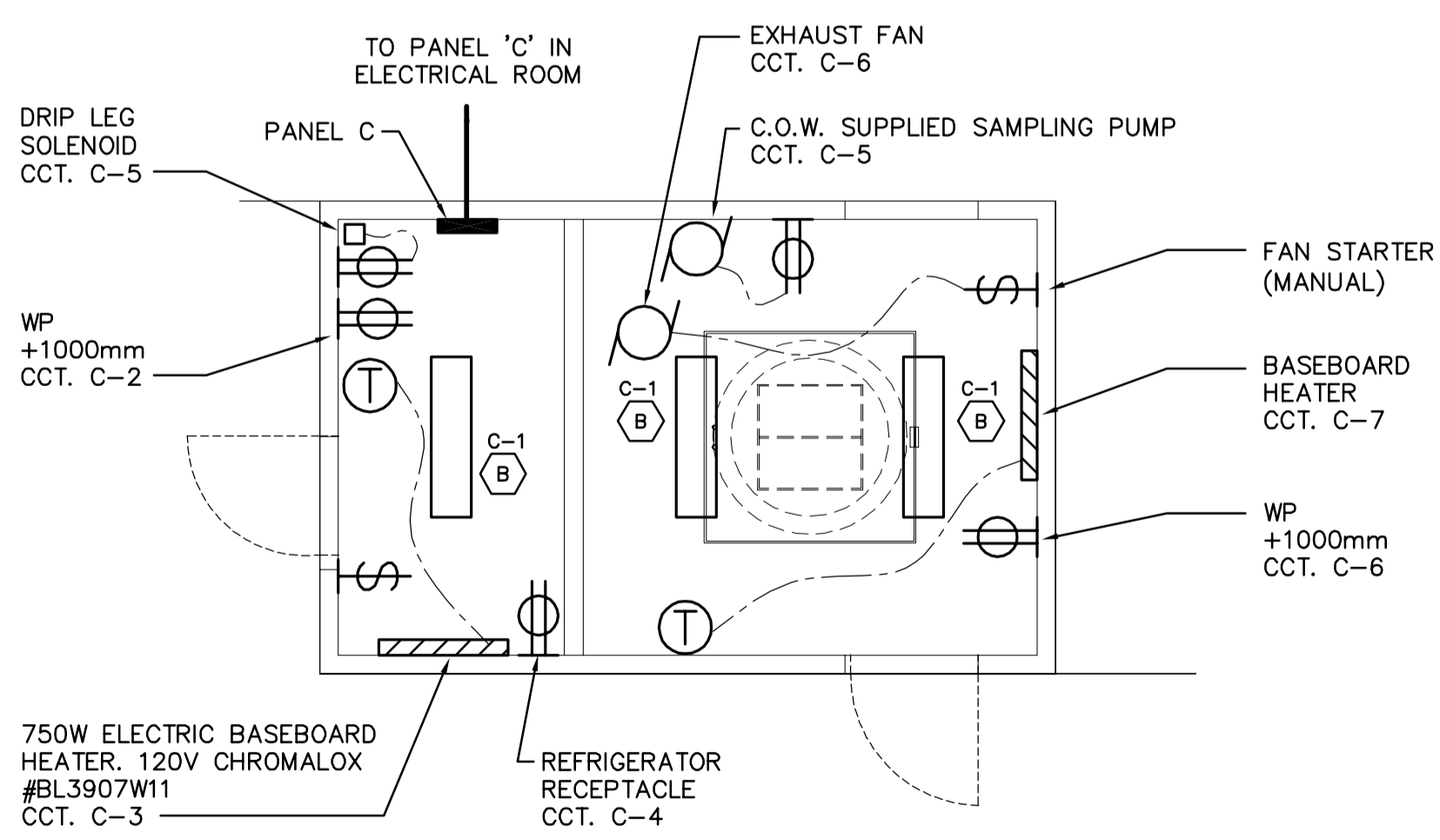
2 EFFLUENT SAMPLING BUILDING ELECTRICAL E1.01 SCALE 1:50
