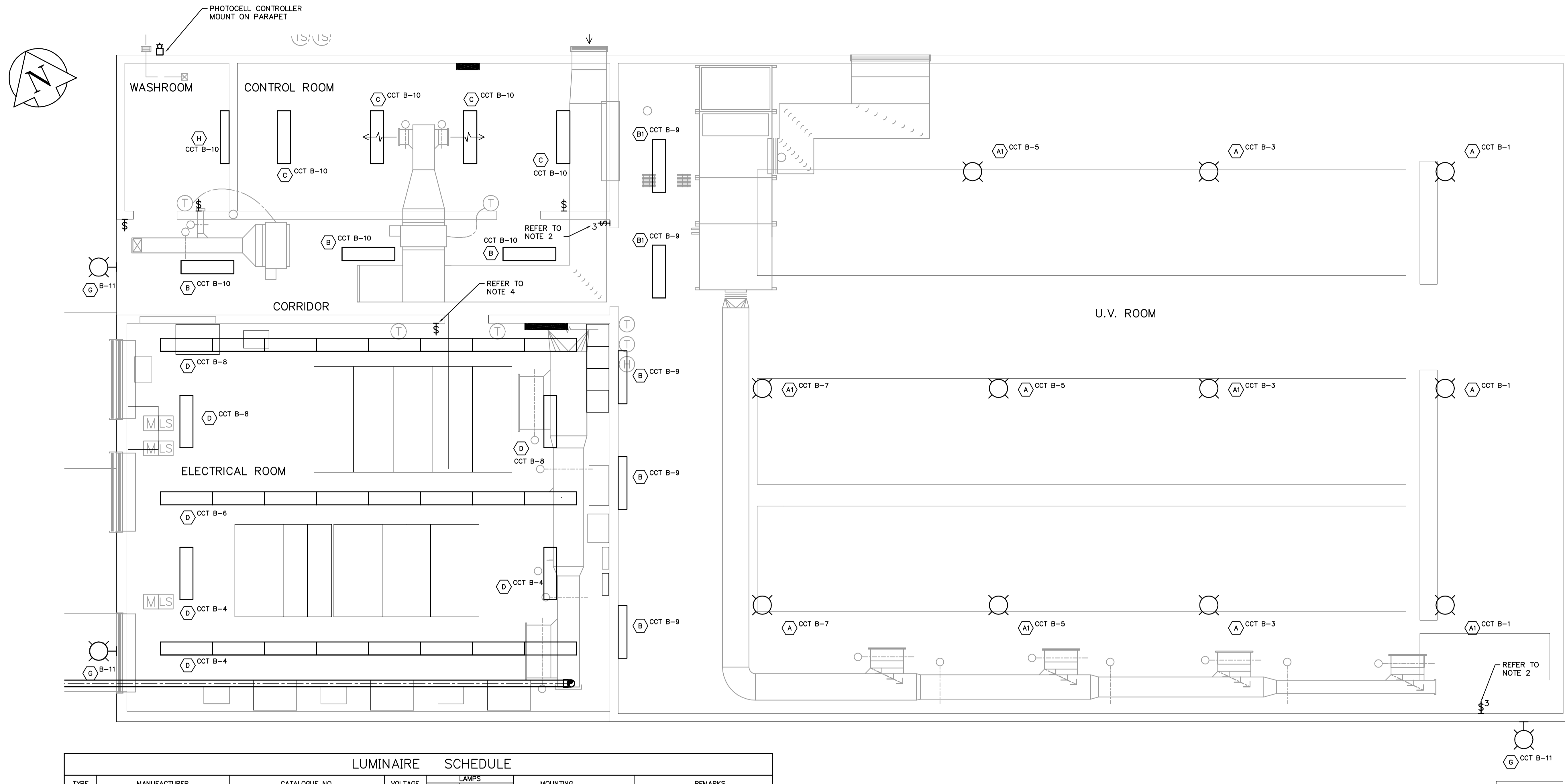
FLOOR PLAN - LIGHTING SCALE 1:50
