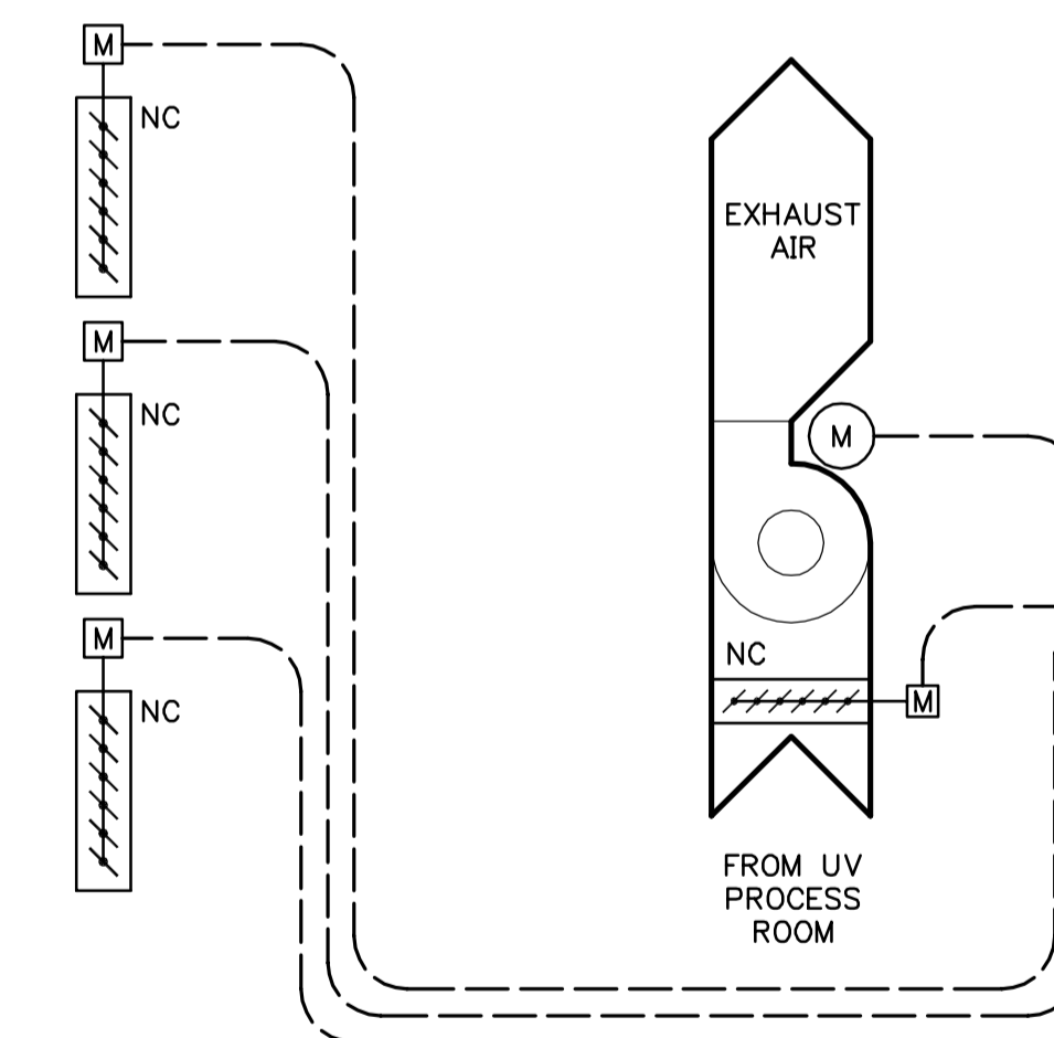
4 U-419-EF EMERGENCY COOLING SYSTEM M8.03 SCALE N.T.S.
