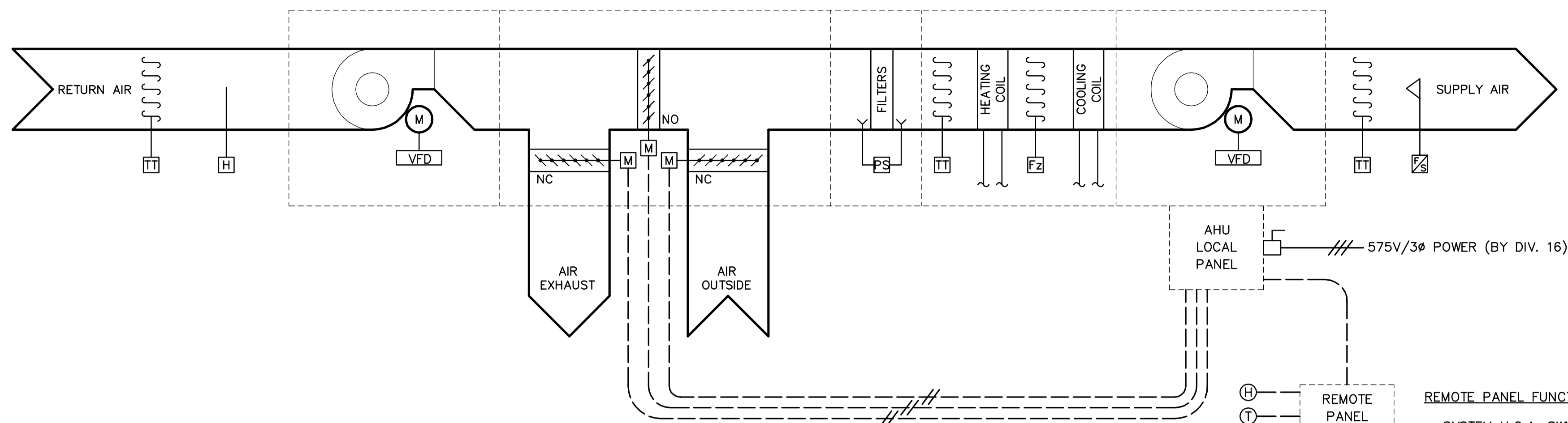
1 U-420-AHU-1 UV PROCESS ROOM M8.03 SCALE N.T.S.
