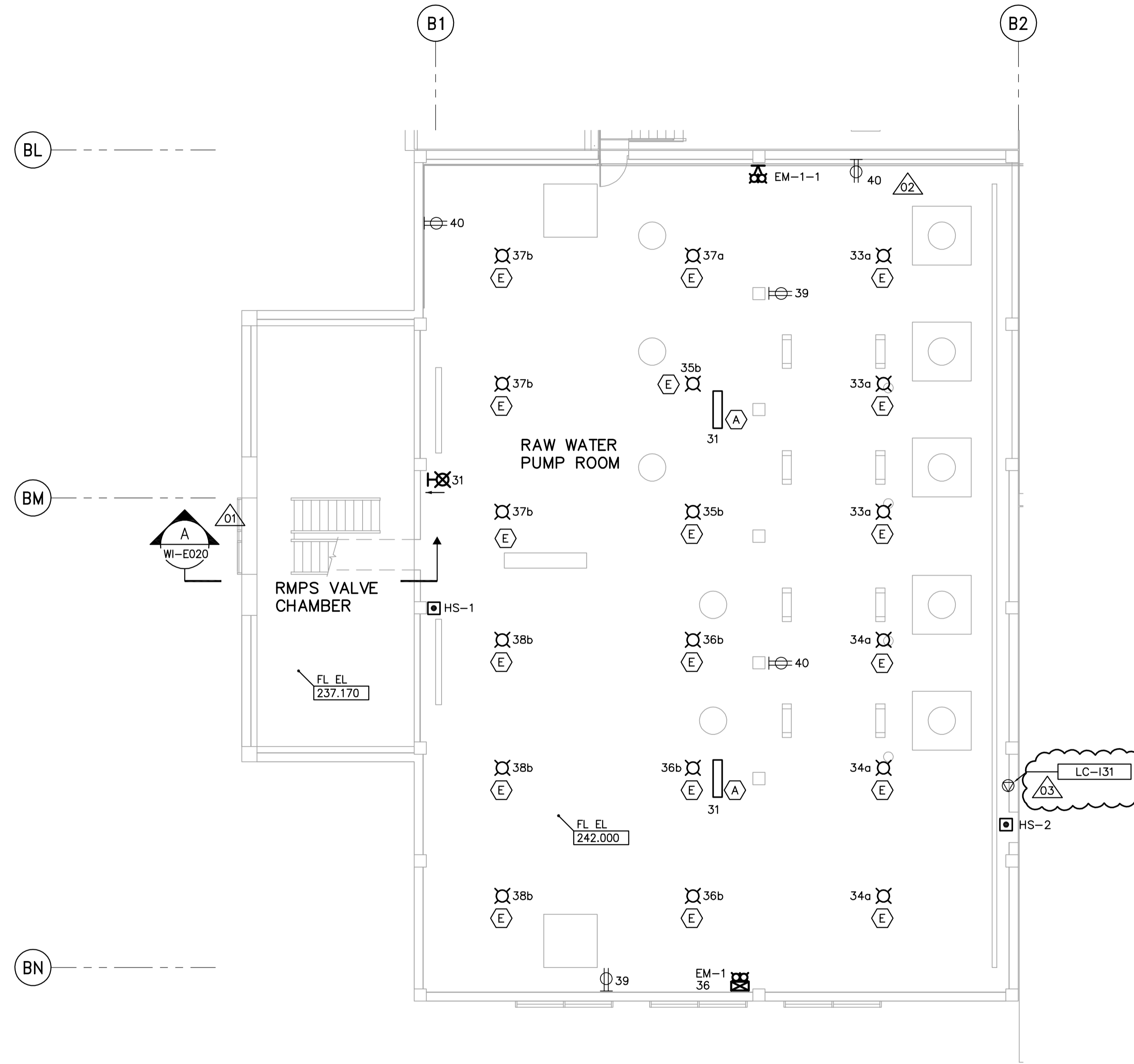
THIRD FLOOR POWER AND LIGHTING PLAN 1:100
