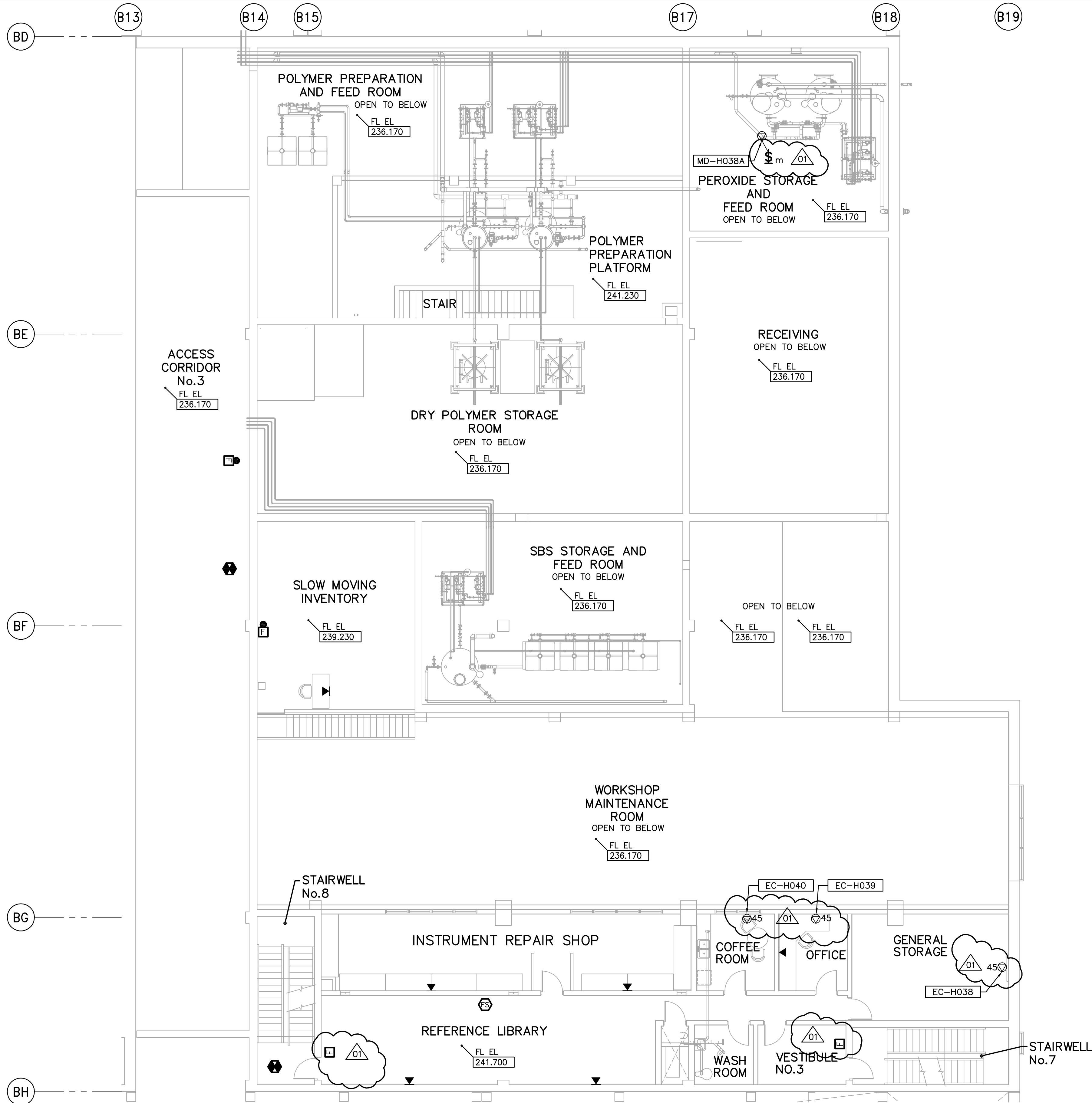
SECOND FLOOR FACILITY PLAN 1:100
