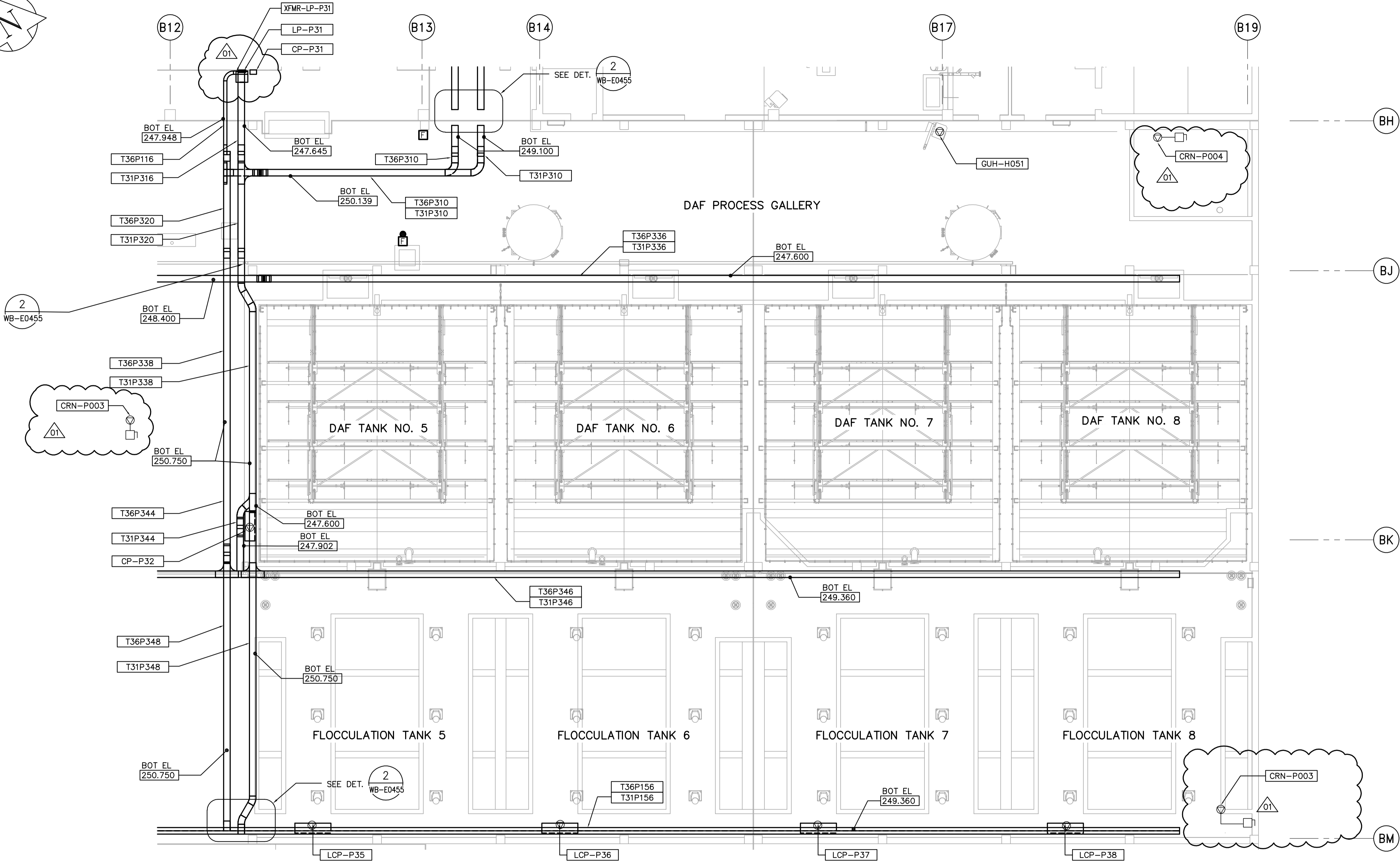
THIRD FLOOR FACILITY PLAN 2 1:100
