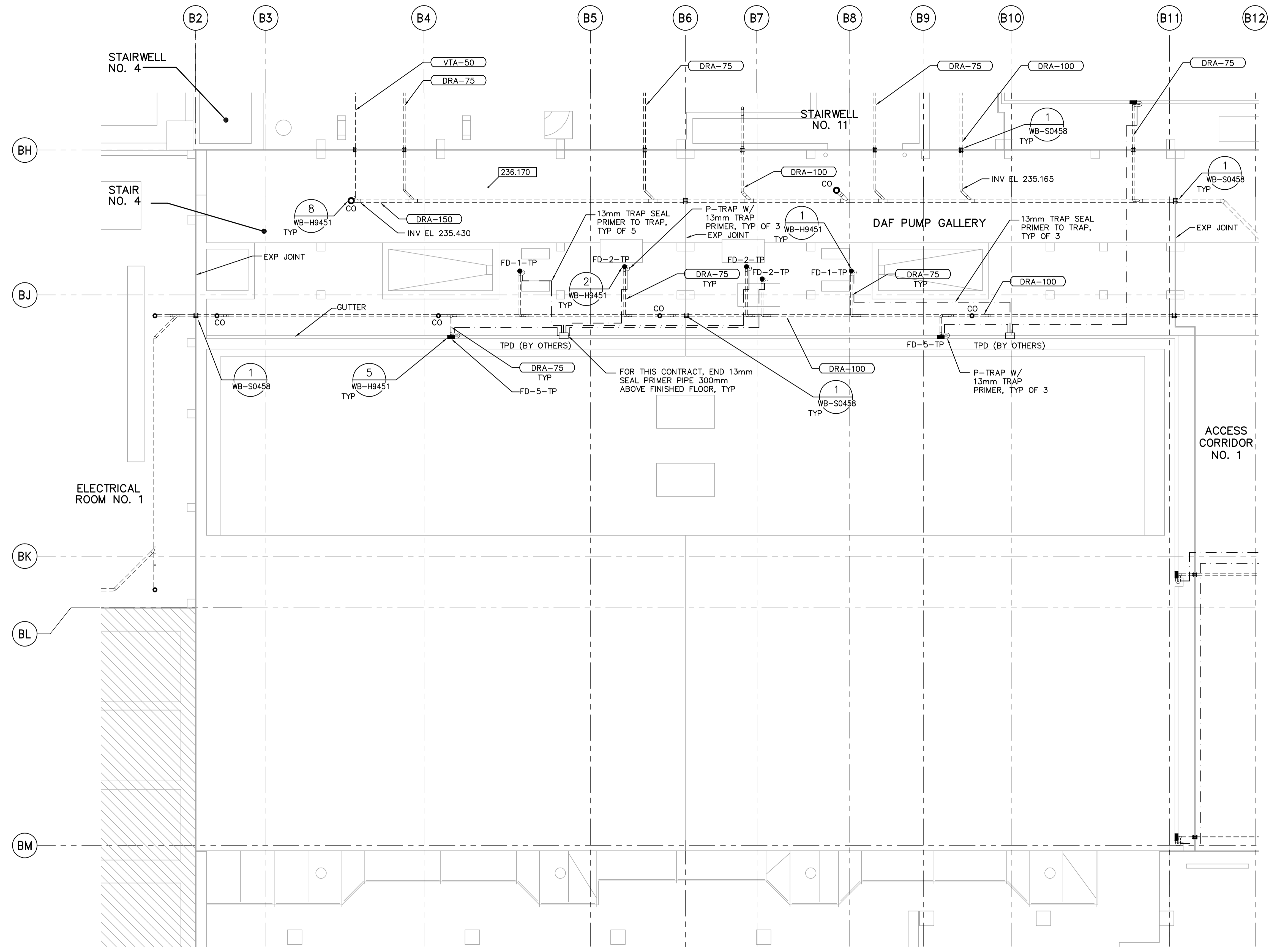
FIRST FLOOR PLAN 1:100
