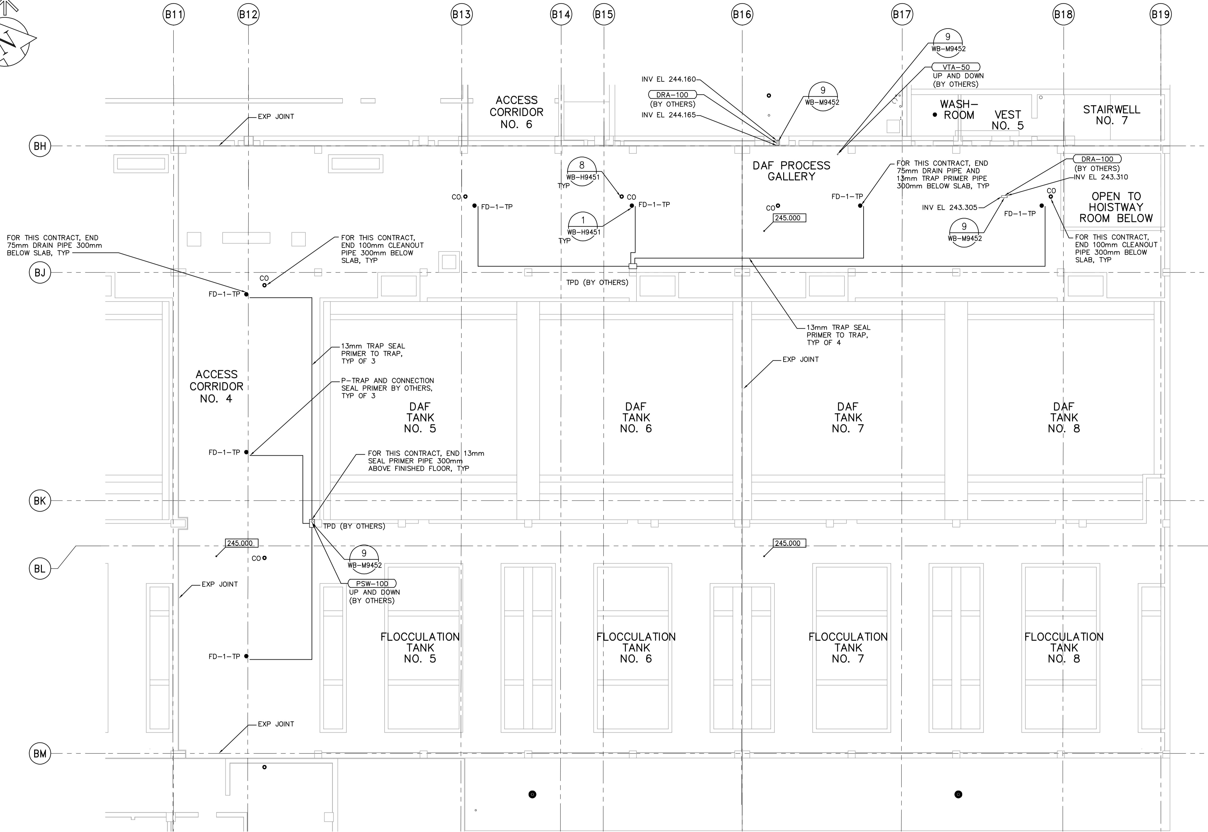
THIRD FLOOR PLAN 1:100
