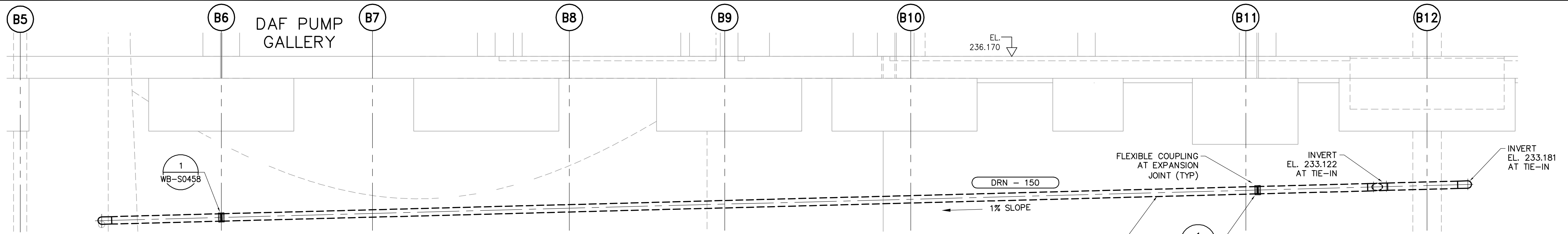
V SECTION - OZONE CONTACTOR DRAIN LINE WP-M9108 1:50
