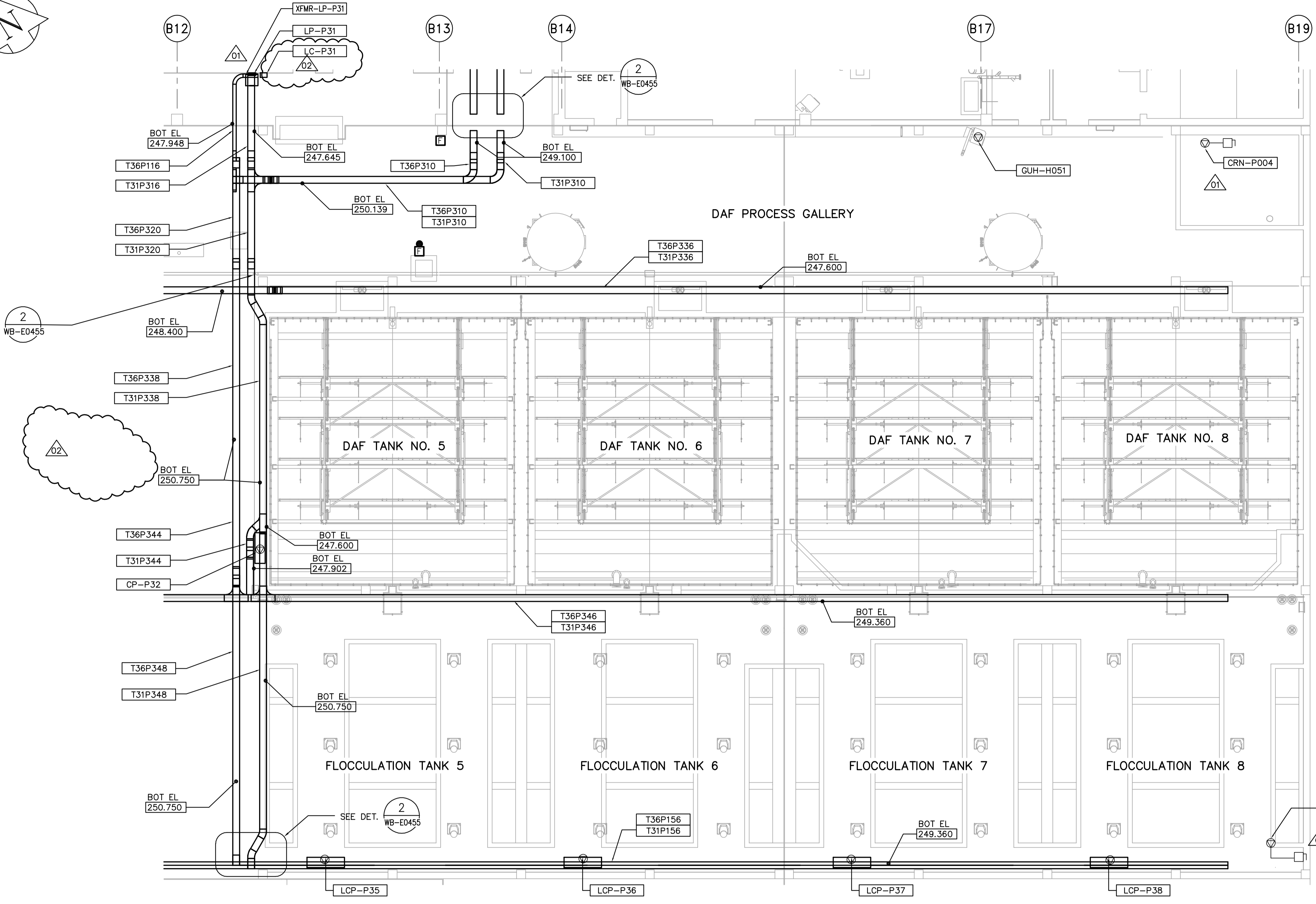
THIRD FLOOR FACILITY PLAN 2 1:100
