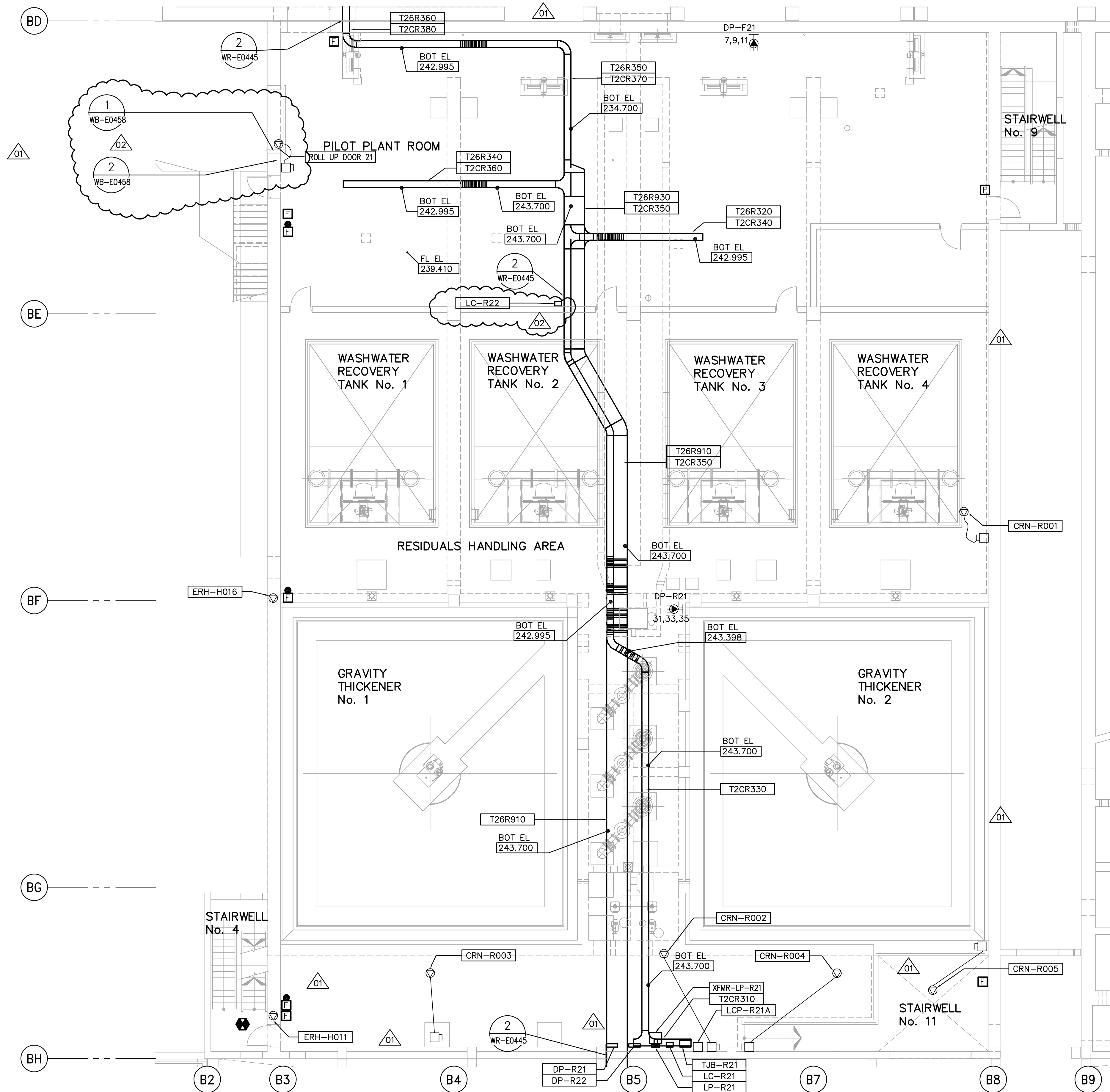
SECOND FLOOR FACILITY PLAN 1:100
