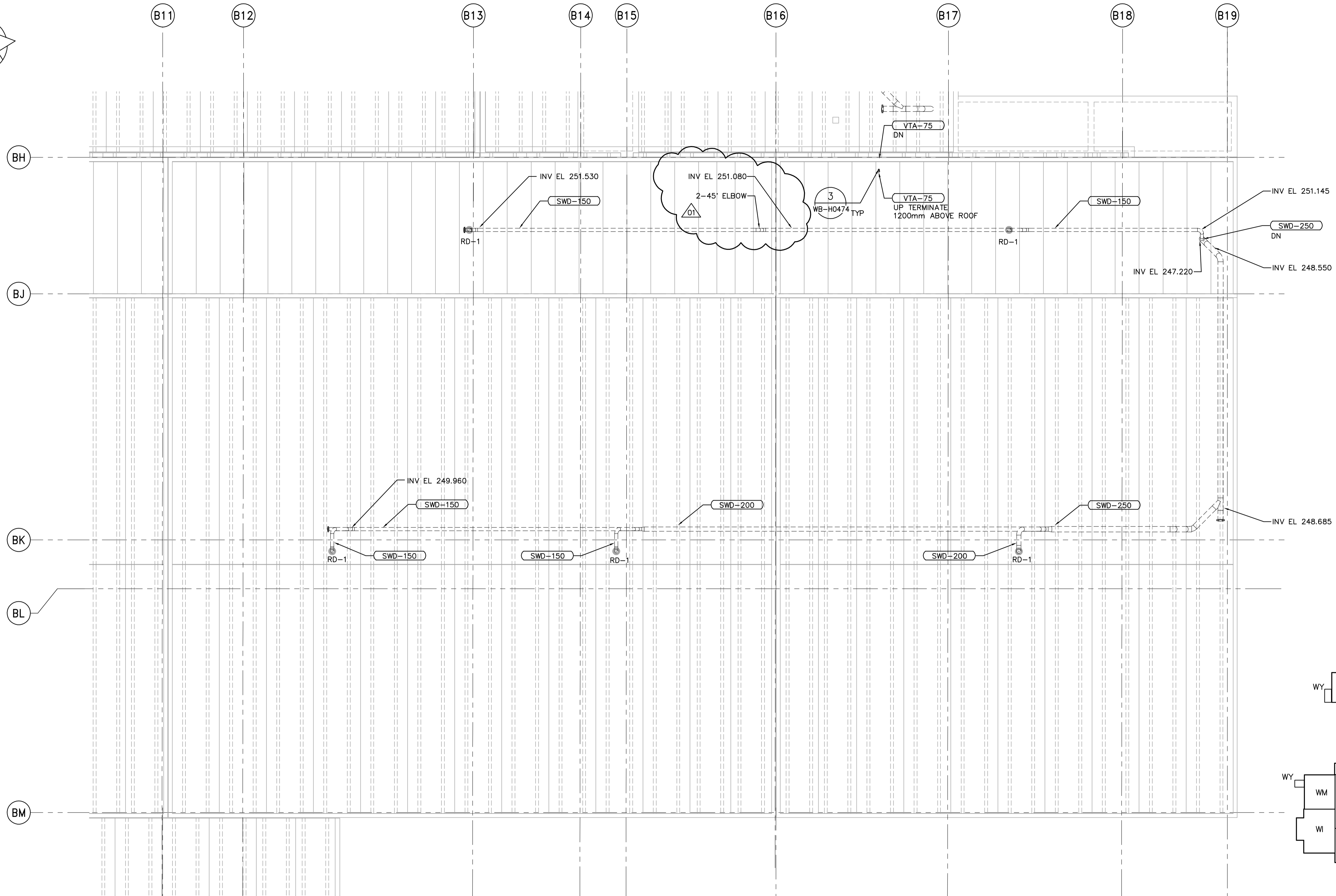
ROOF PLAN 1:100
