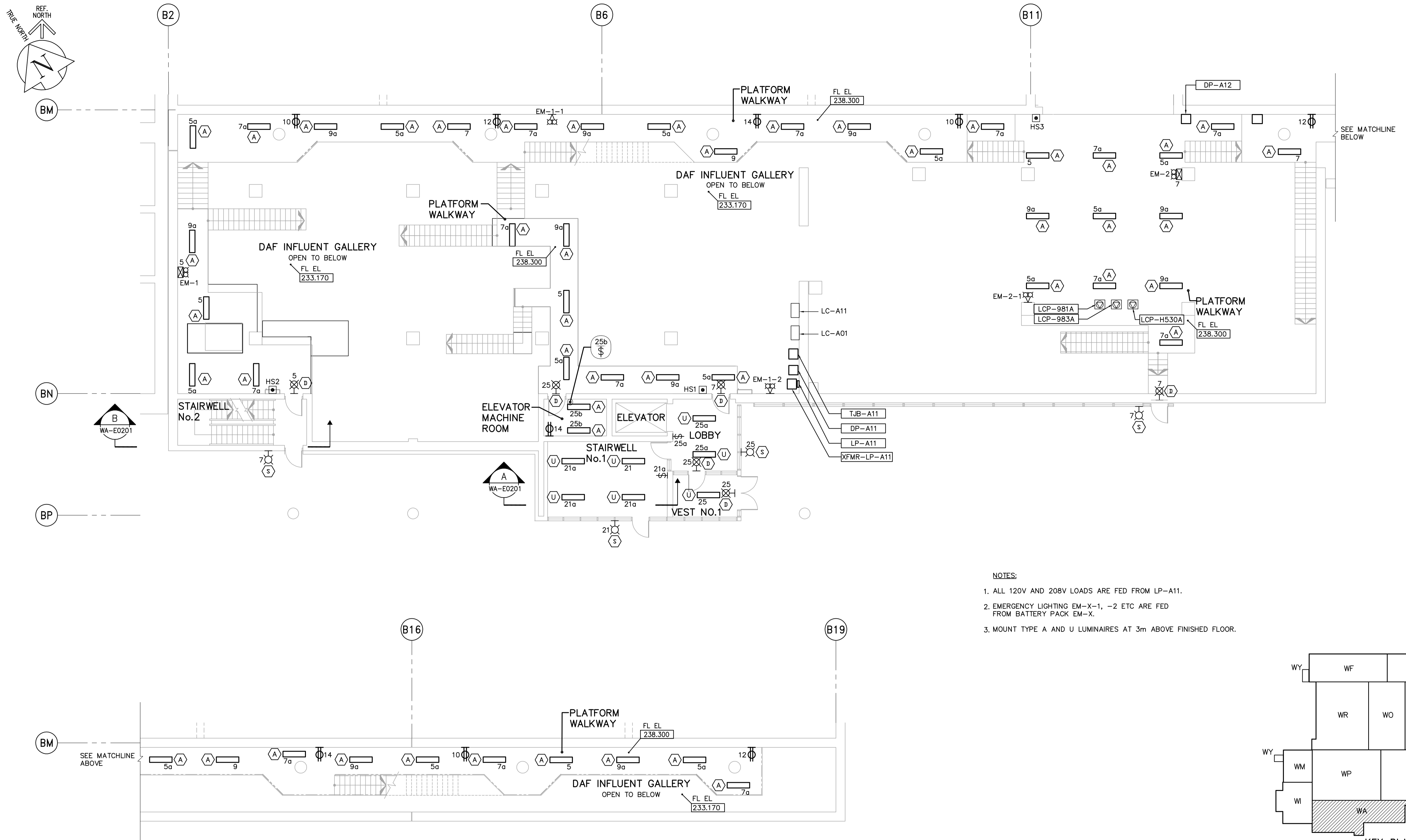
FIRST FLOOR POWER AND LIGHTING PLAN 1:100
