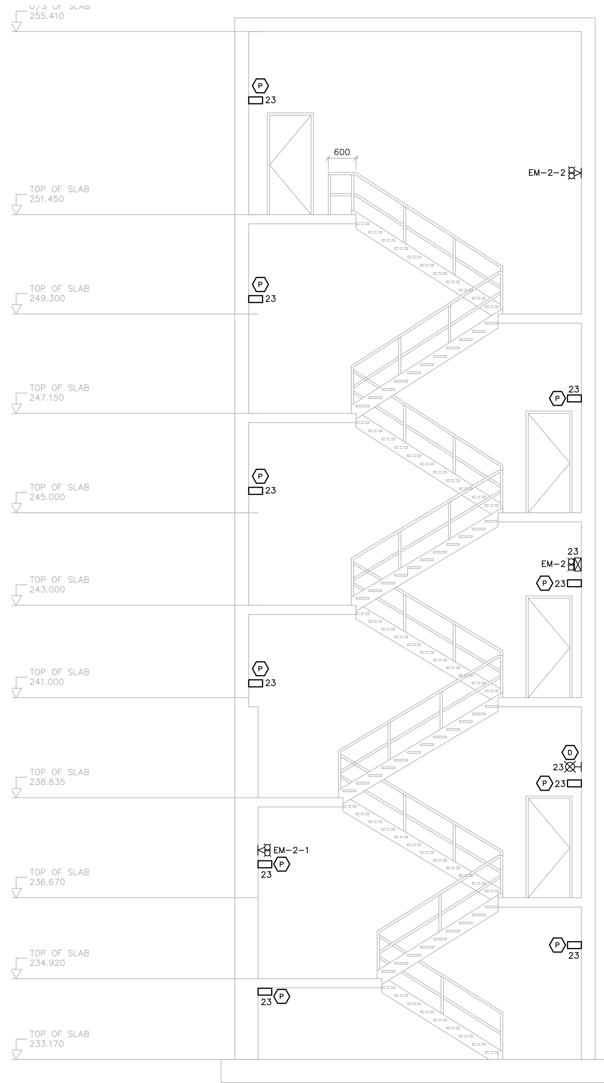
B STAIRWELL No.2 LIGHTING WA-E0123 1:50 WA-E0402 WA-E0113
