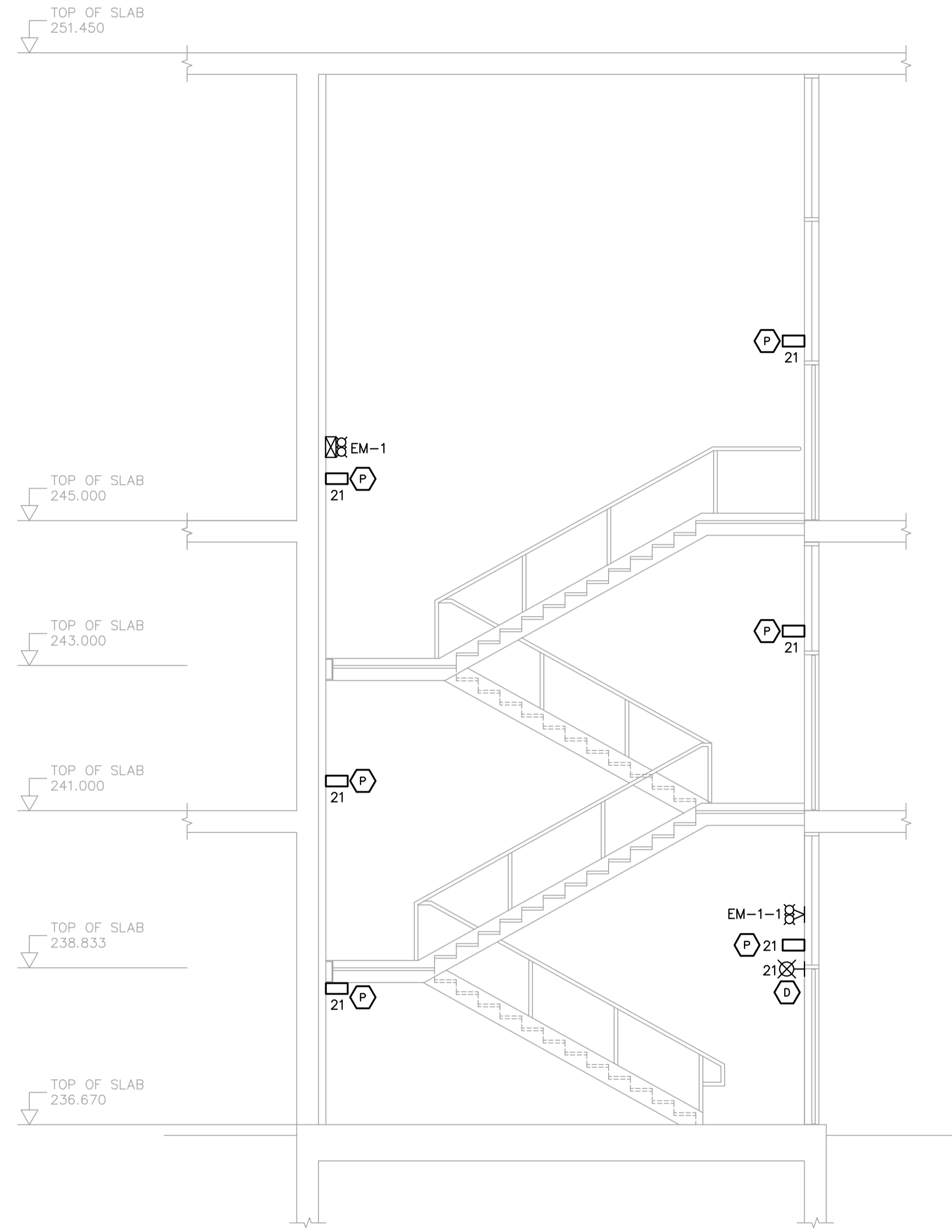
A STAIRWELL No.1 LIGHTING WA-E0123 1:50 WA-E0402 WA-E0103 WA-E0113
