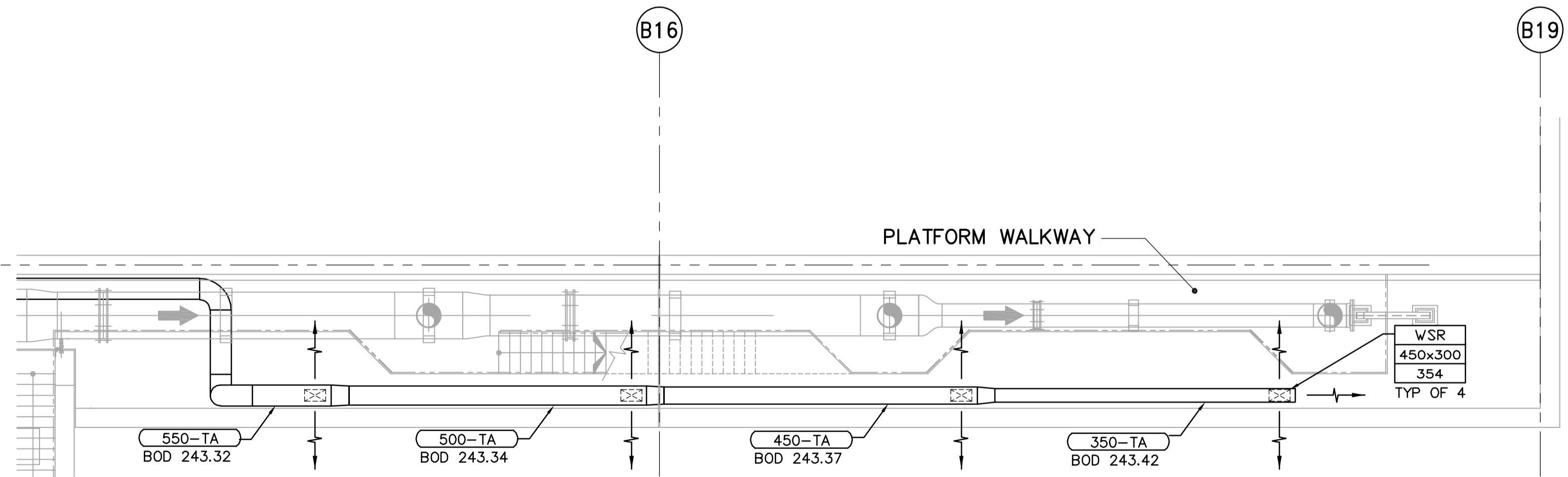
FIRST FLOOR PLAN 1:100
