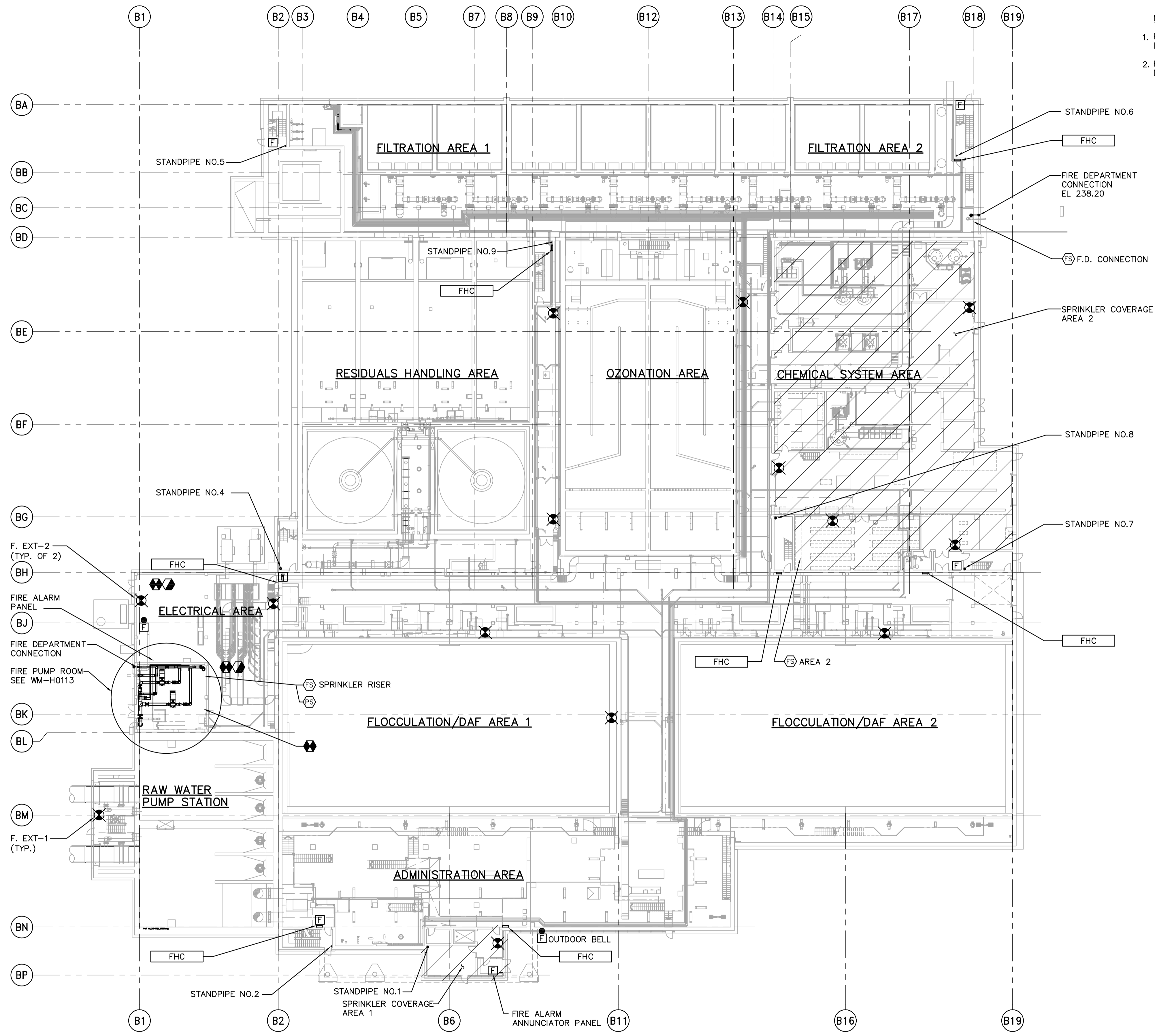
FIRST FLOOR PLAN 1:300
