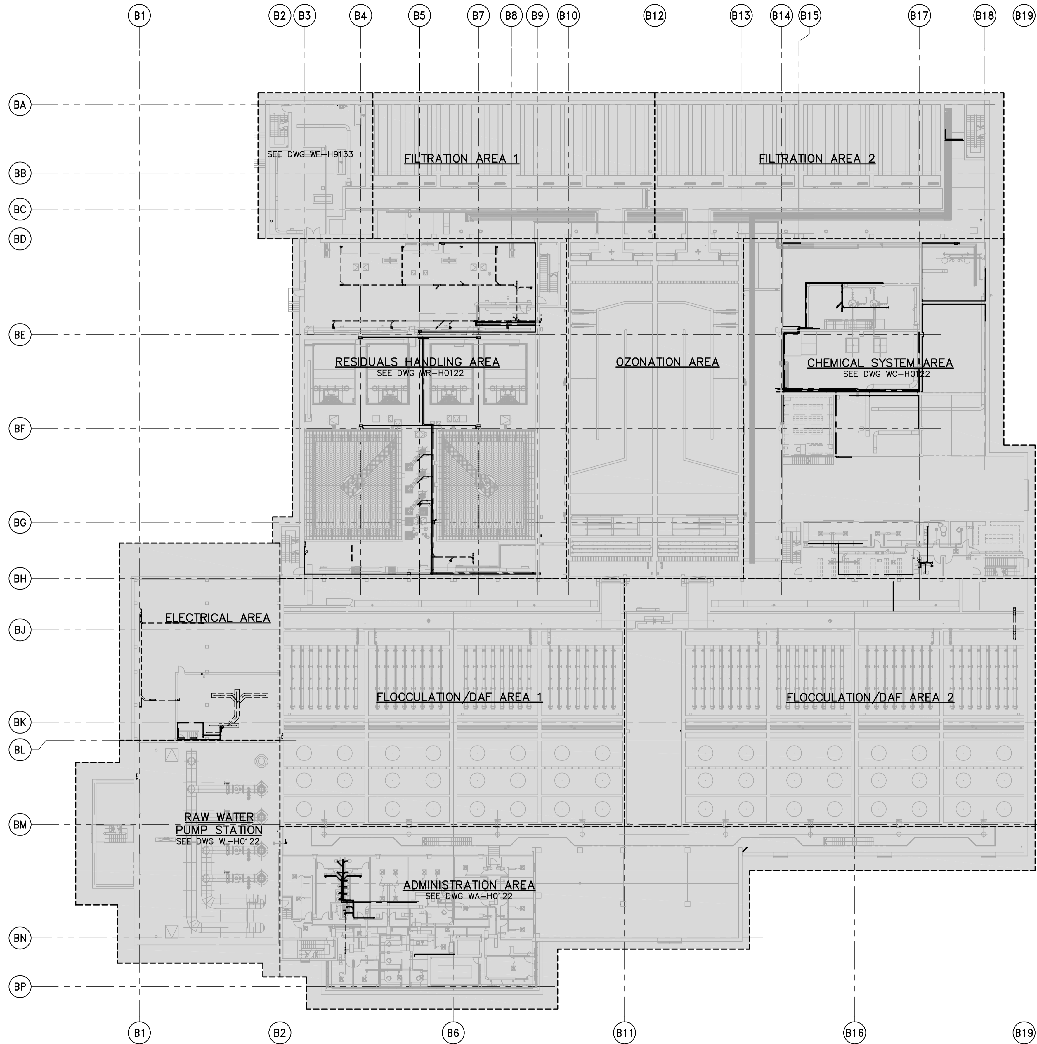
SECOND FLOOR KEY PLAN 1:100
