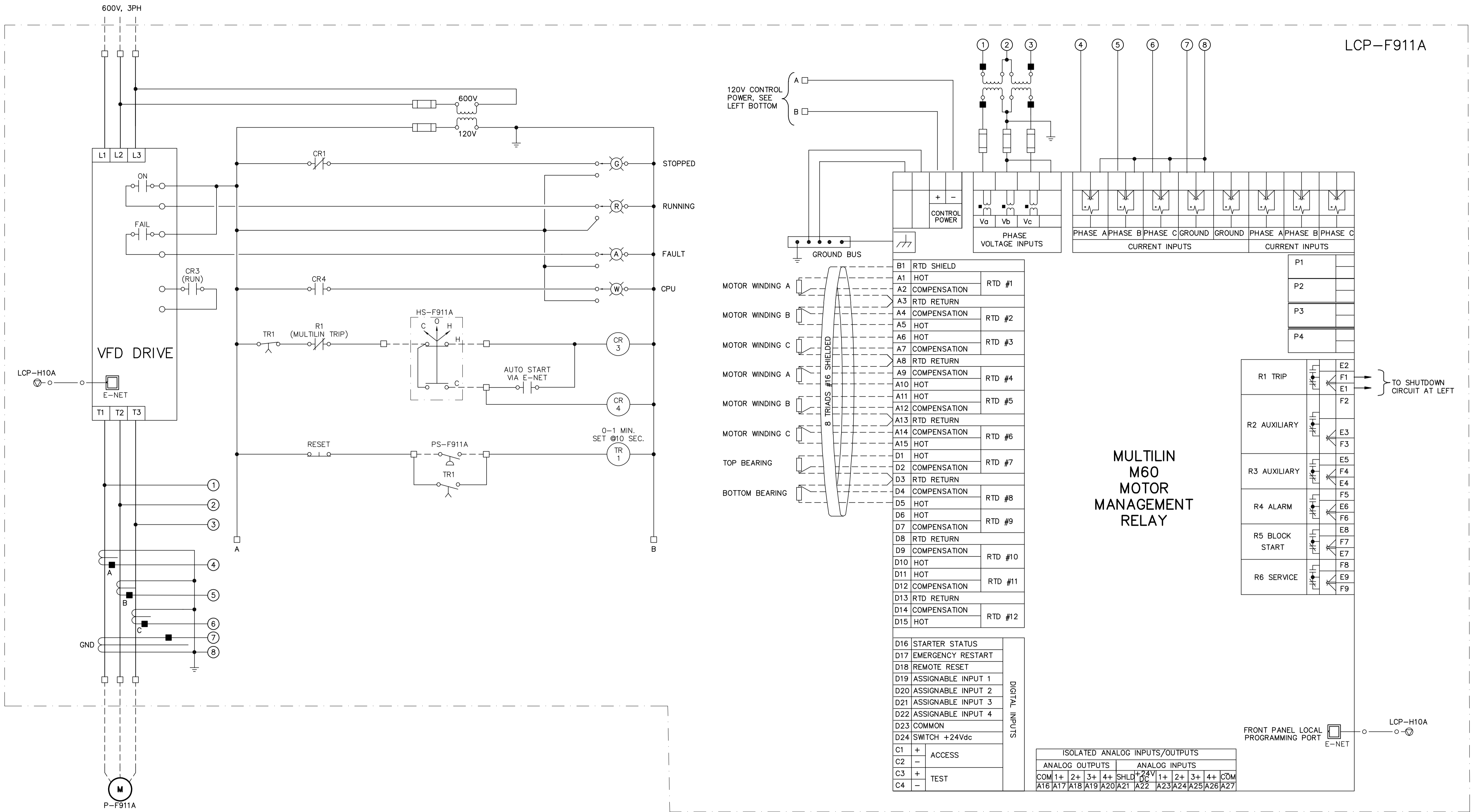
BACKWASH SUPPLY PUMP (P-F911A)
