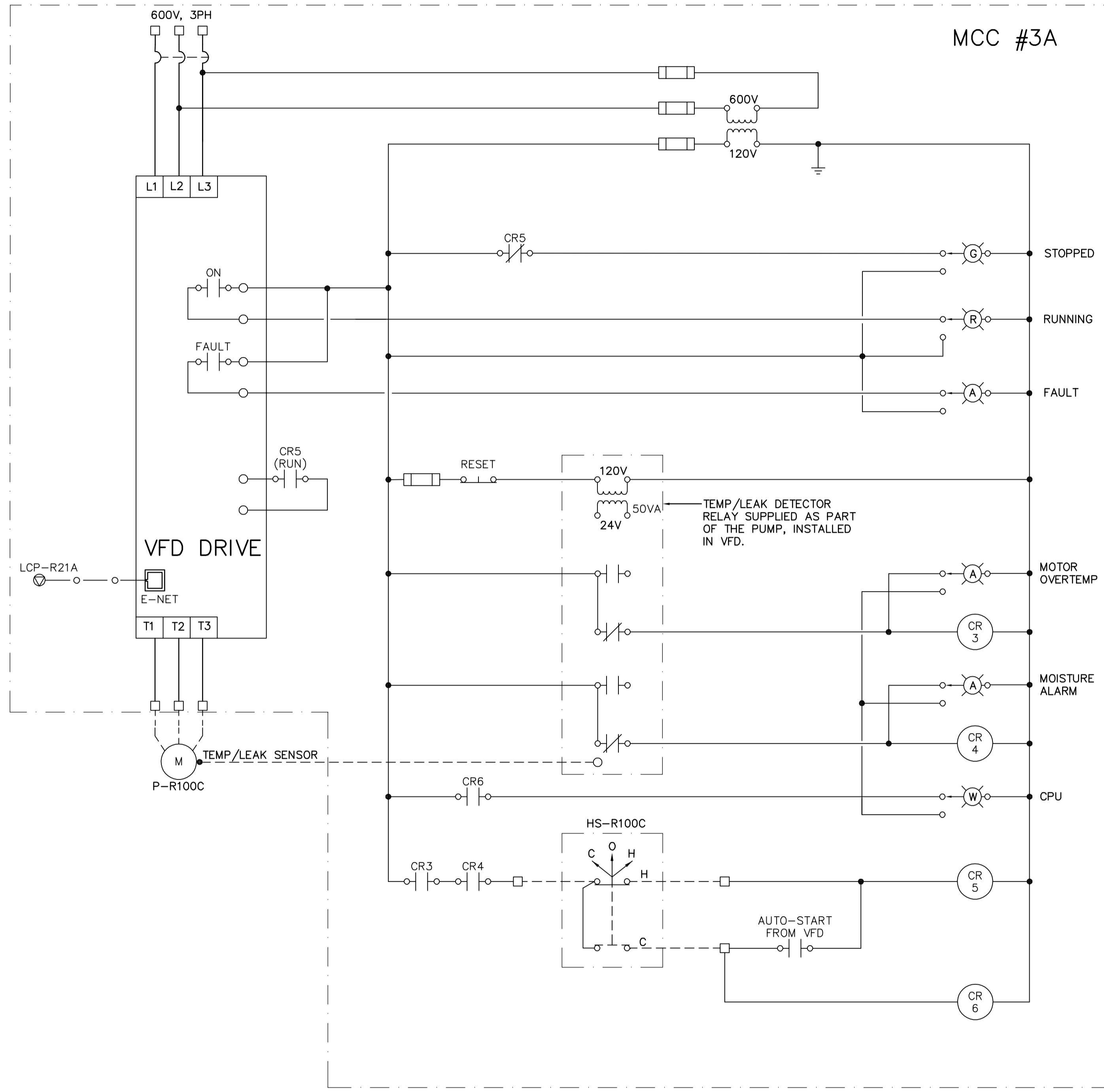
SLUDGE PUMP (P-R100C)
