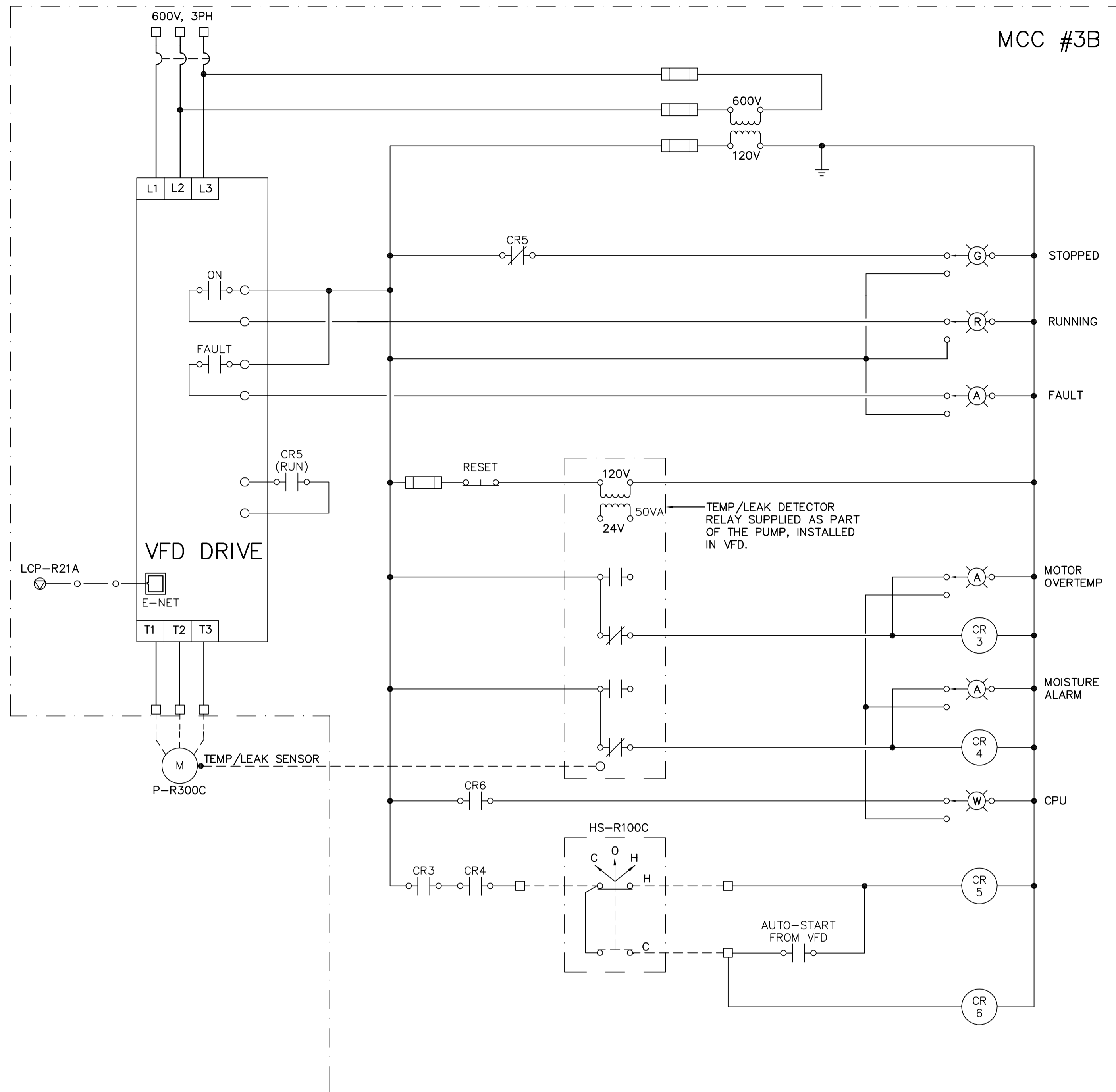
SLUDGE PUMP (P-R300C)
