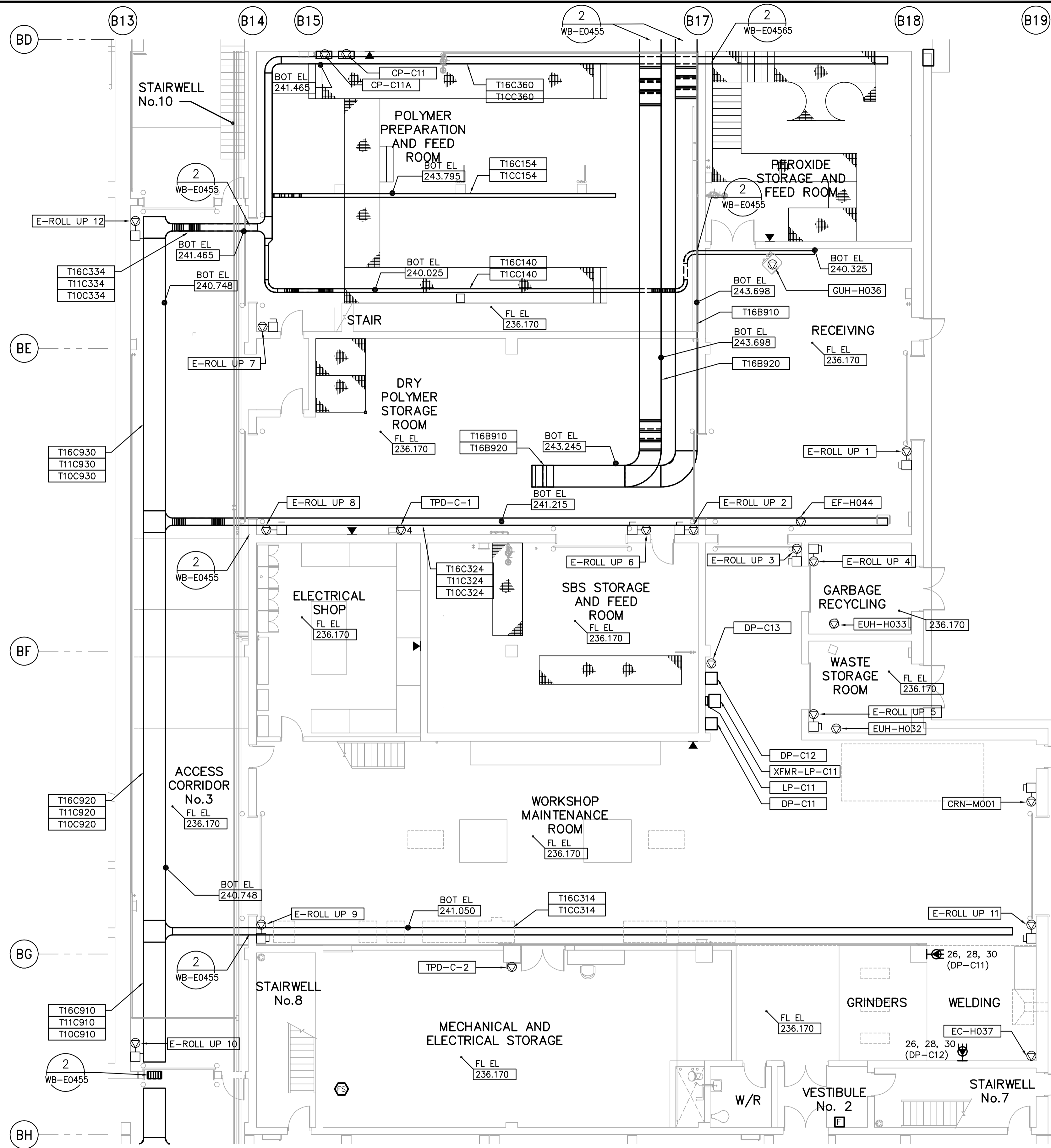
FIRST FLOOR FACILITY PLAN 1:100
