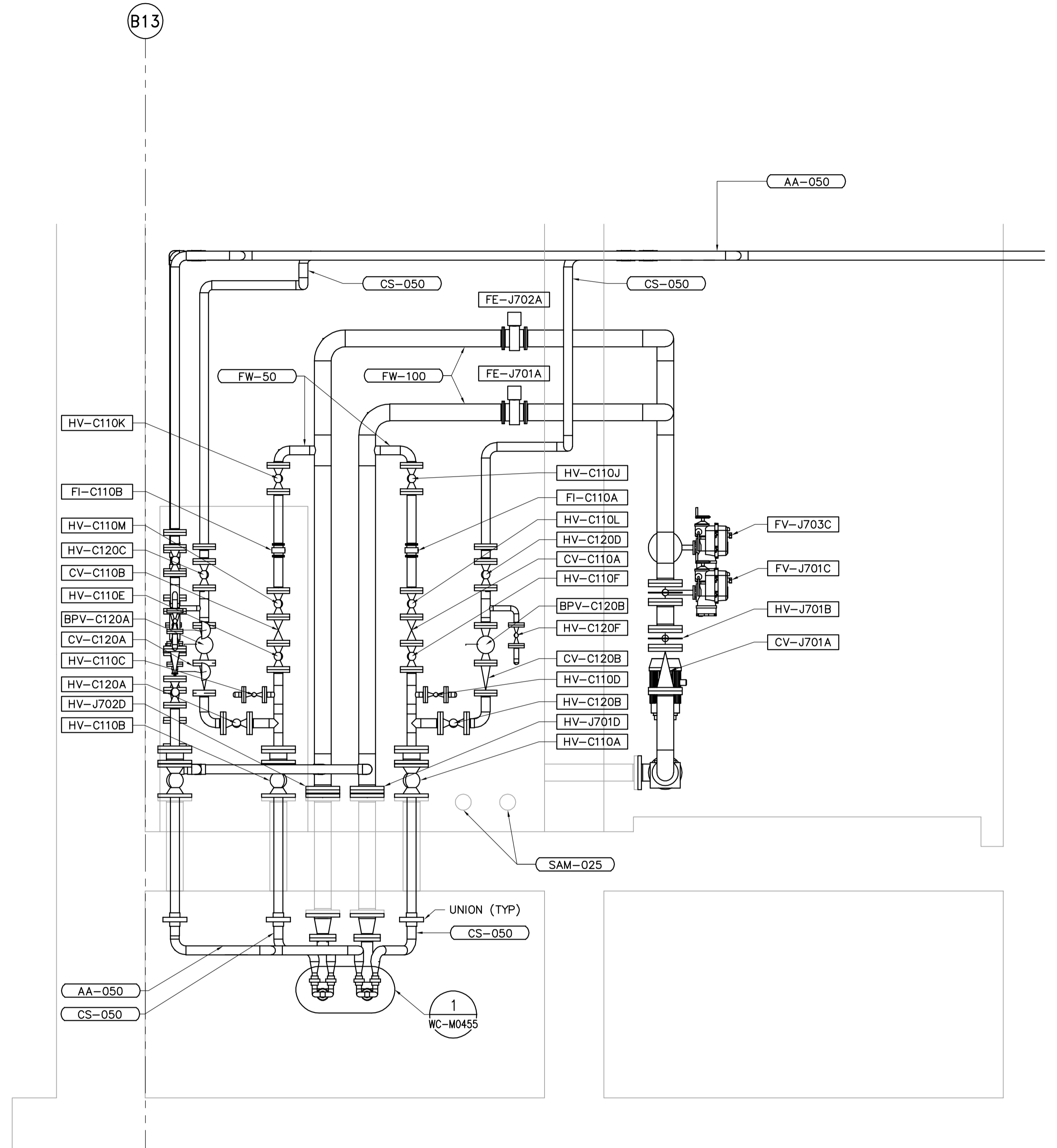
F DETAIL WF-M0401 1:20
