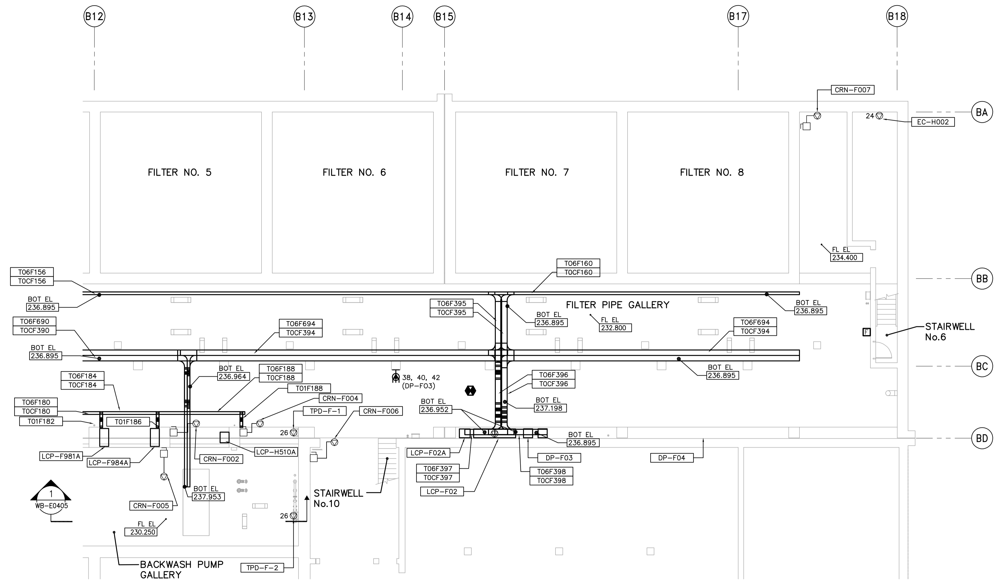
LOWER LEVEL FACILITY PLAN (AREA 2) 1:100
