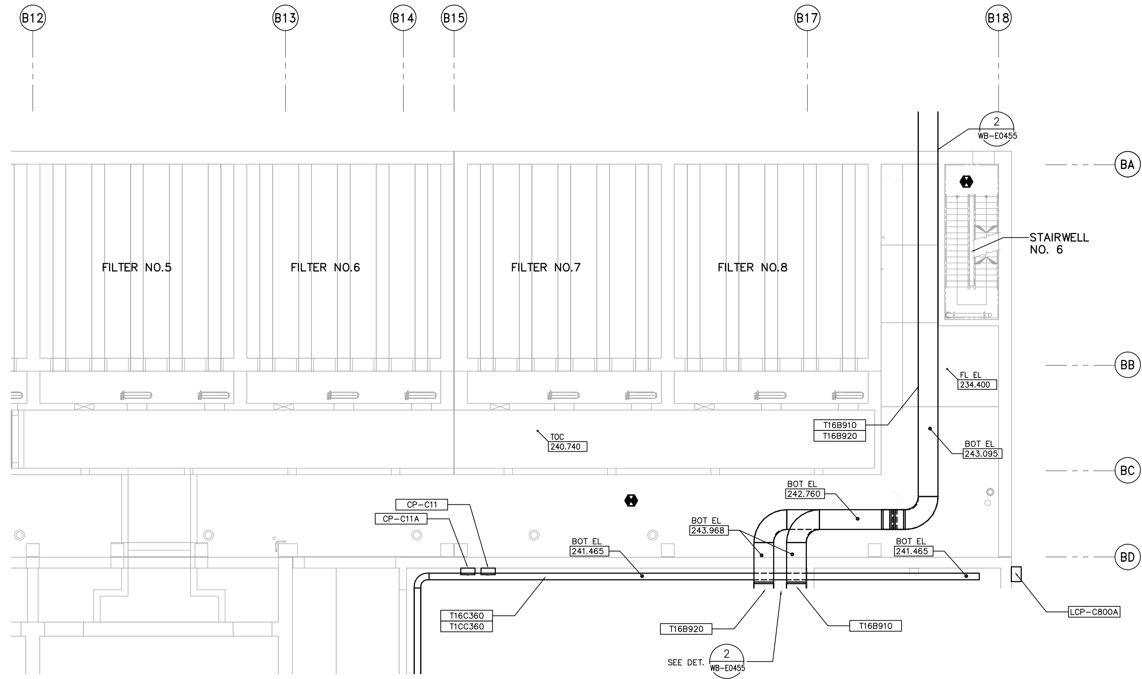
UPPER CHANNEL PLAN 2 1:100
