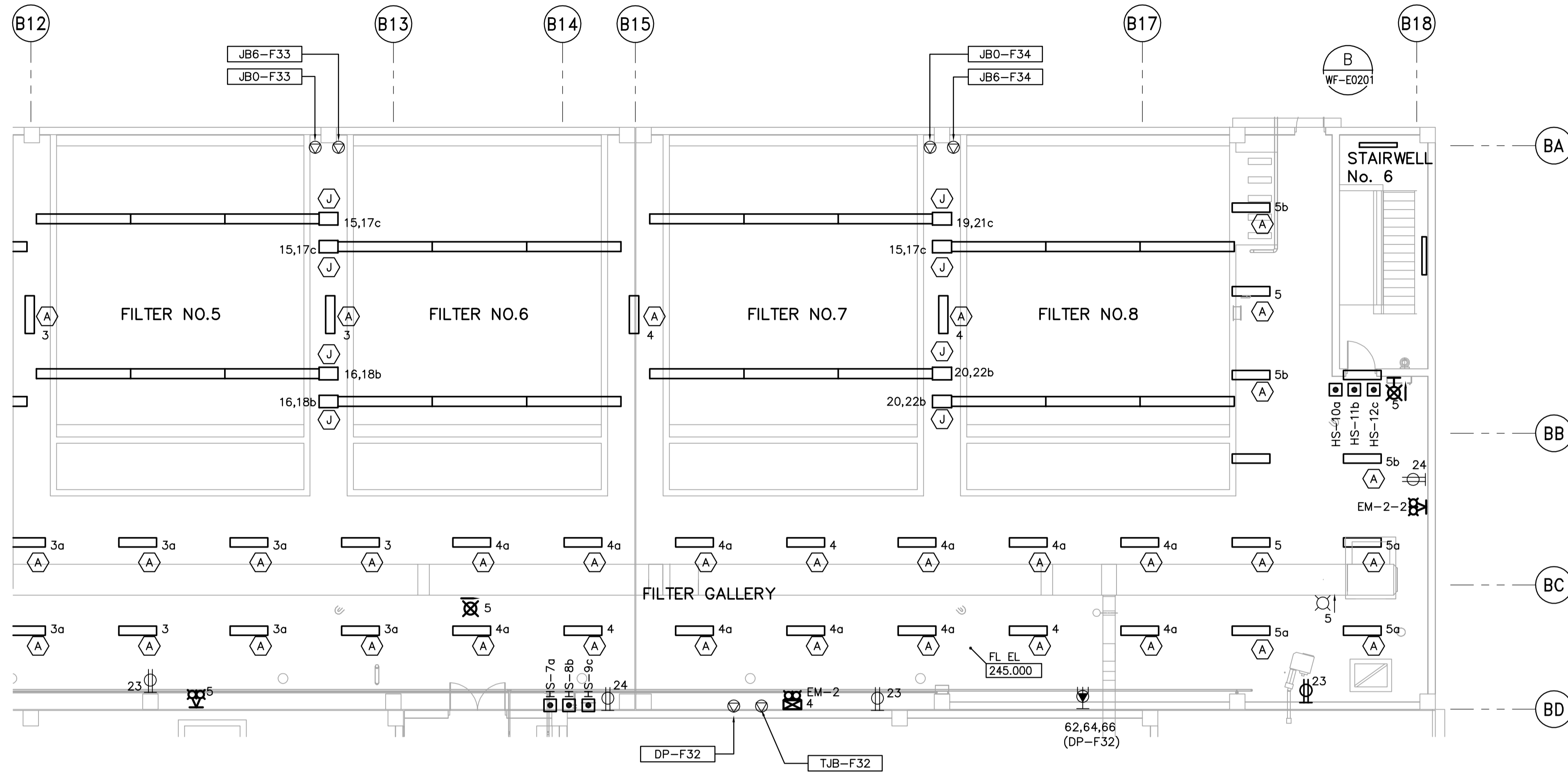
THIRD FLOOR POWER AND LIGHTING PLAN (AREA 2) 1:100
