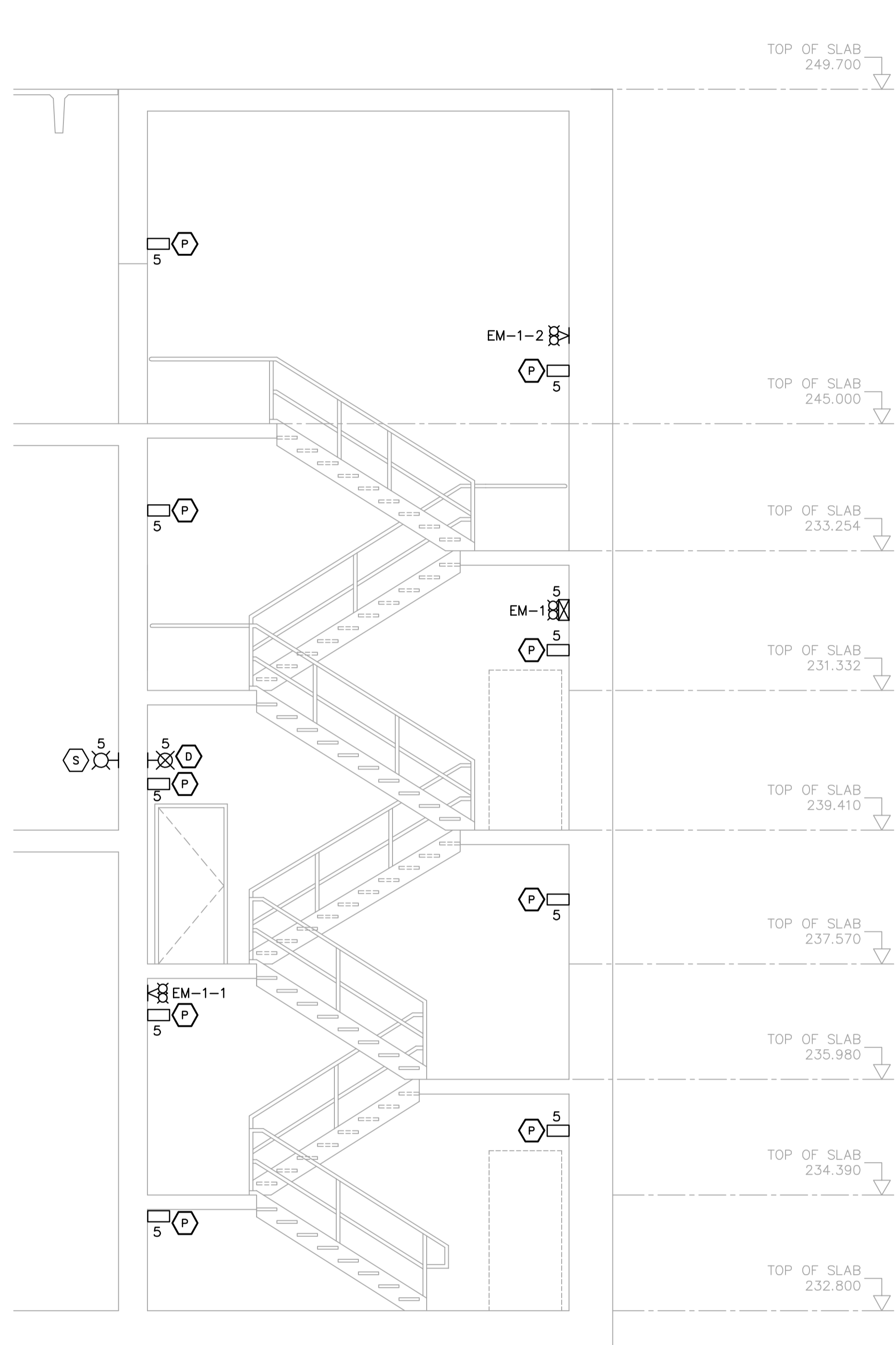
A STAIRWELL NO.5 LIGHTING WF-E0105 1:50 WF-E0125 WF-E0135
