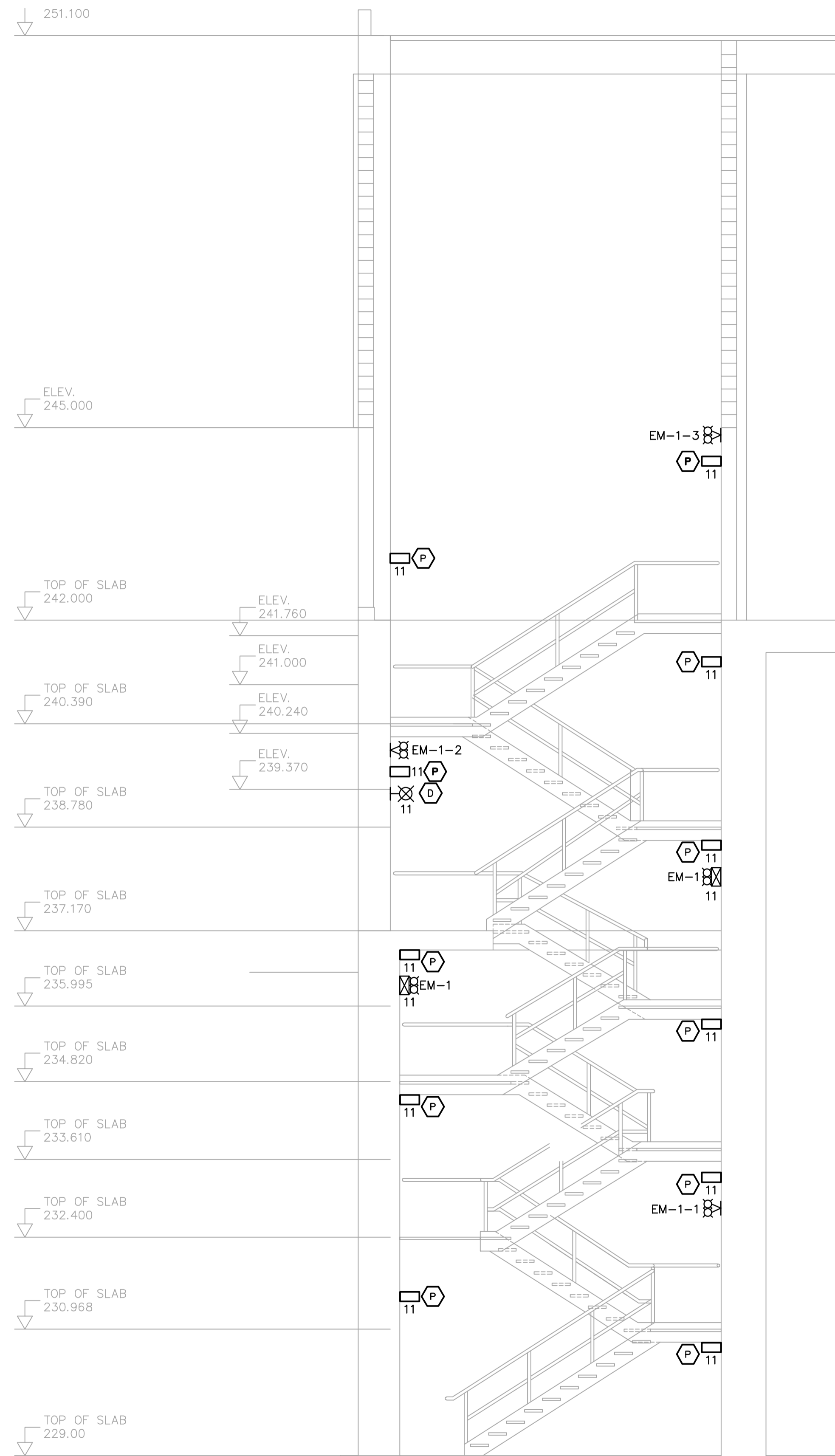
A STAIRWELL NO.3 LIGHTING WI-E0103 1:50 WI-E0113
