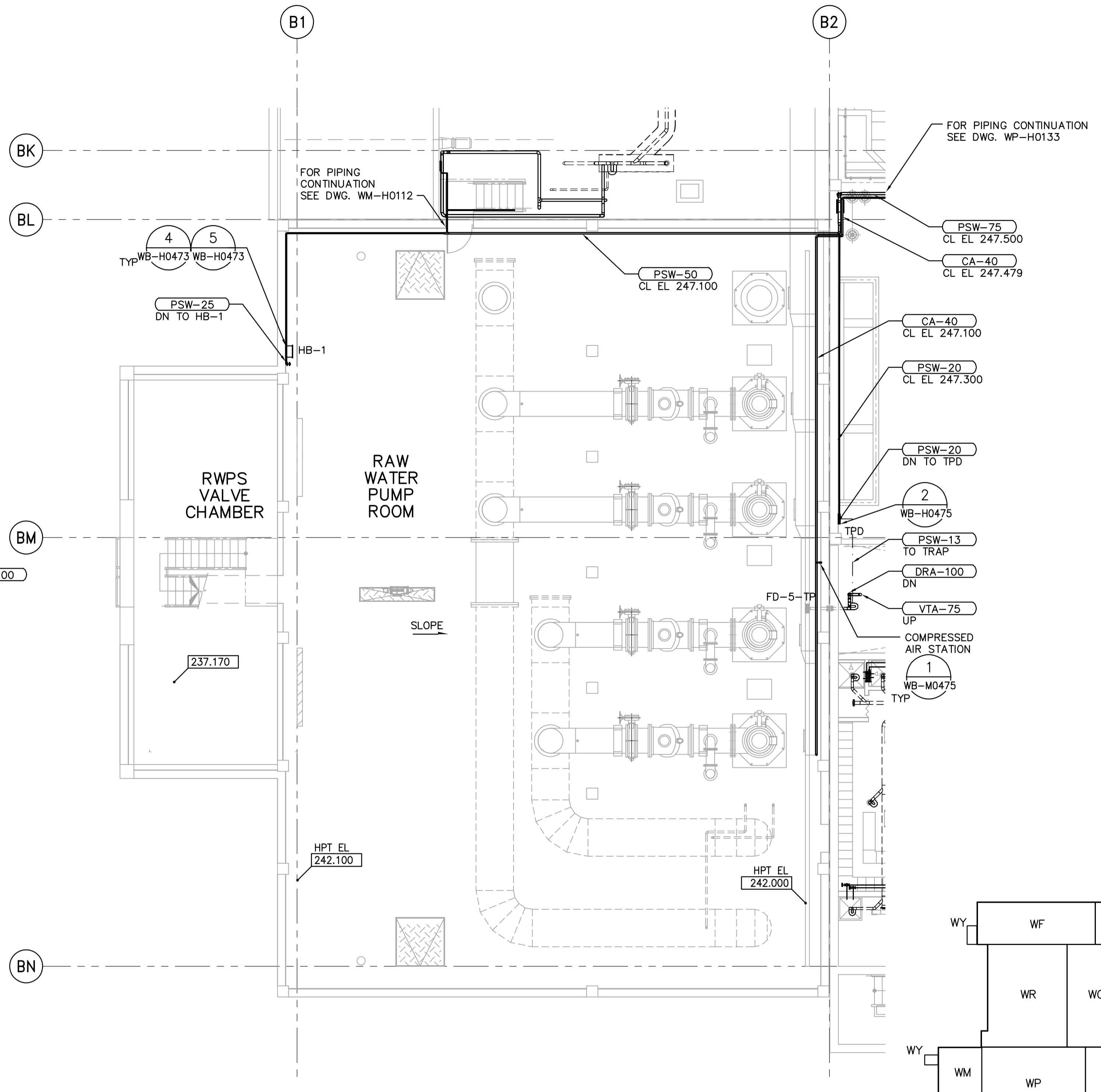
THIRD FLOOR PLAN 1:100
