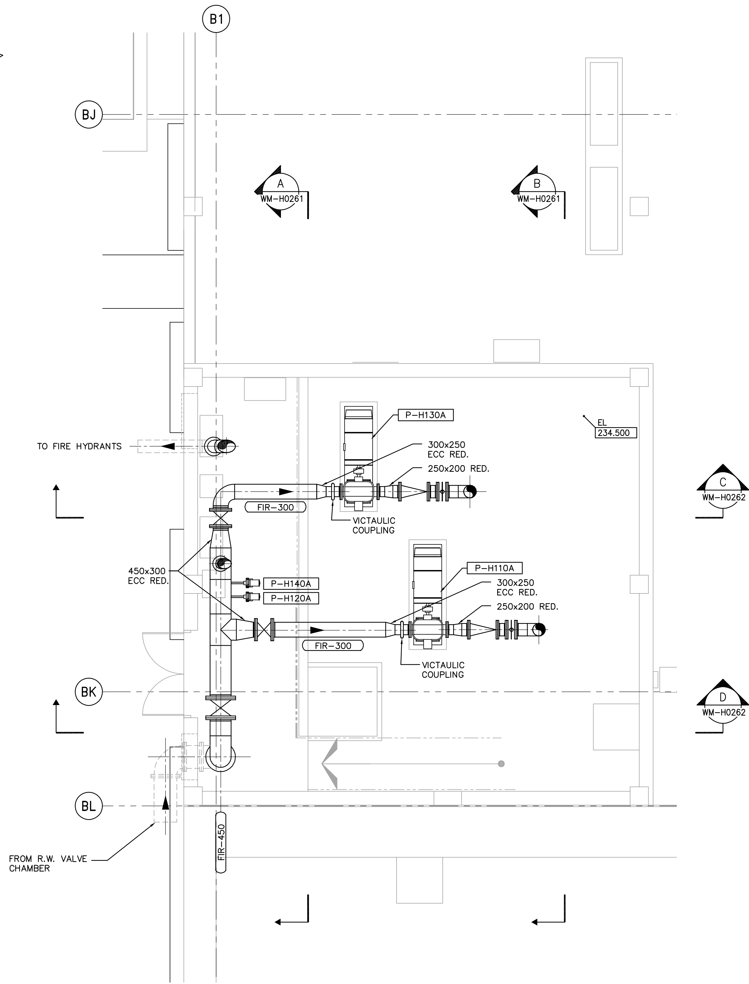
LOWER LEVEL PLAN 1:50
