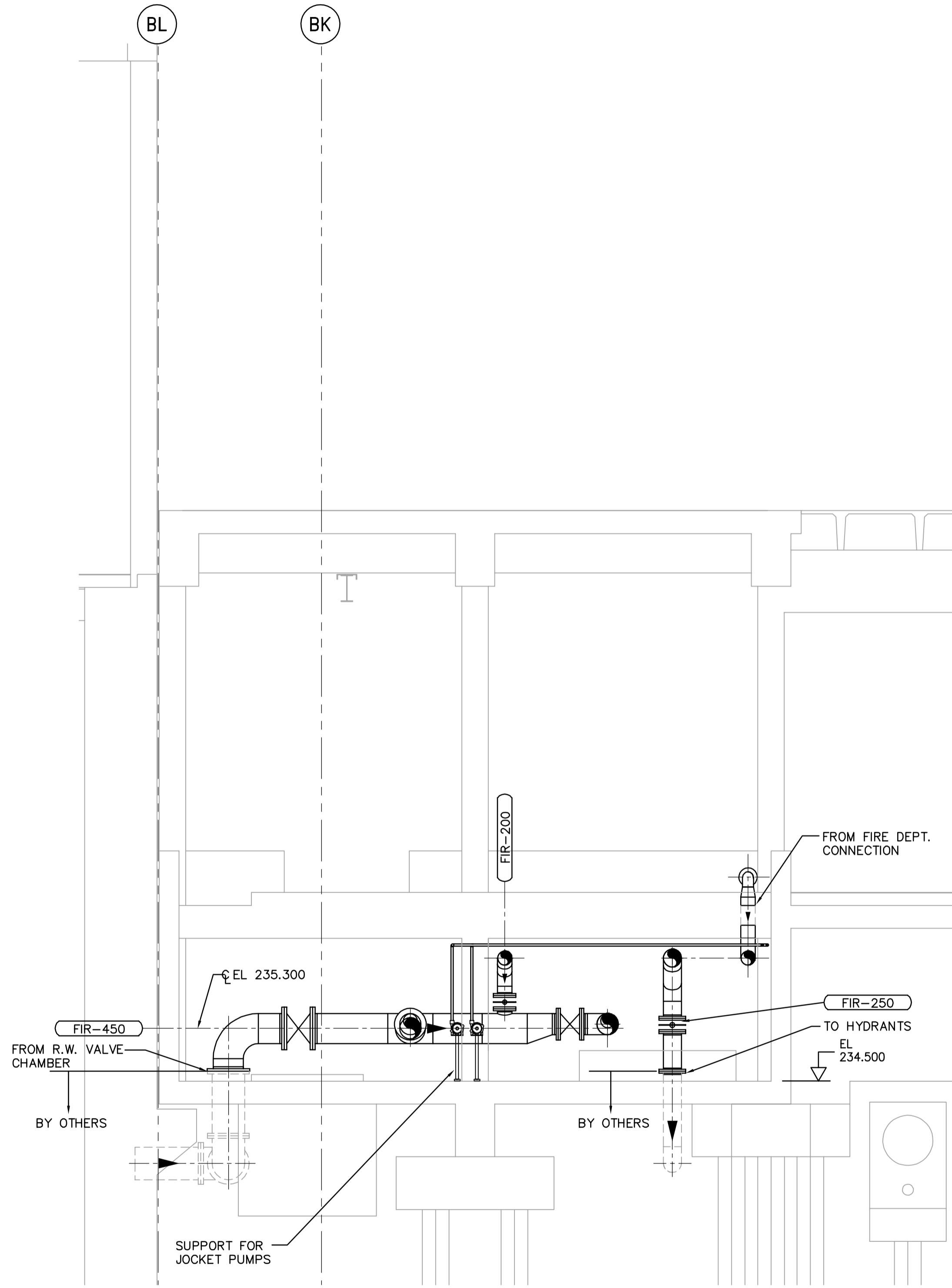
A SECTION WM-H0113 1:50
