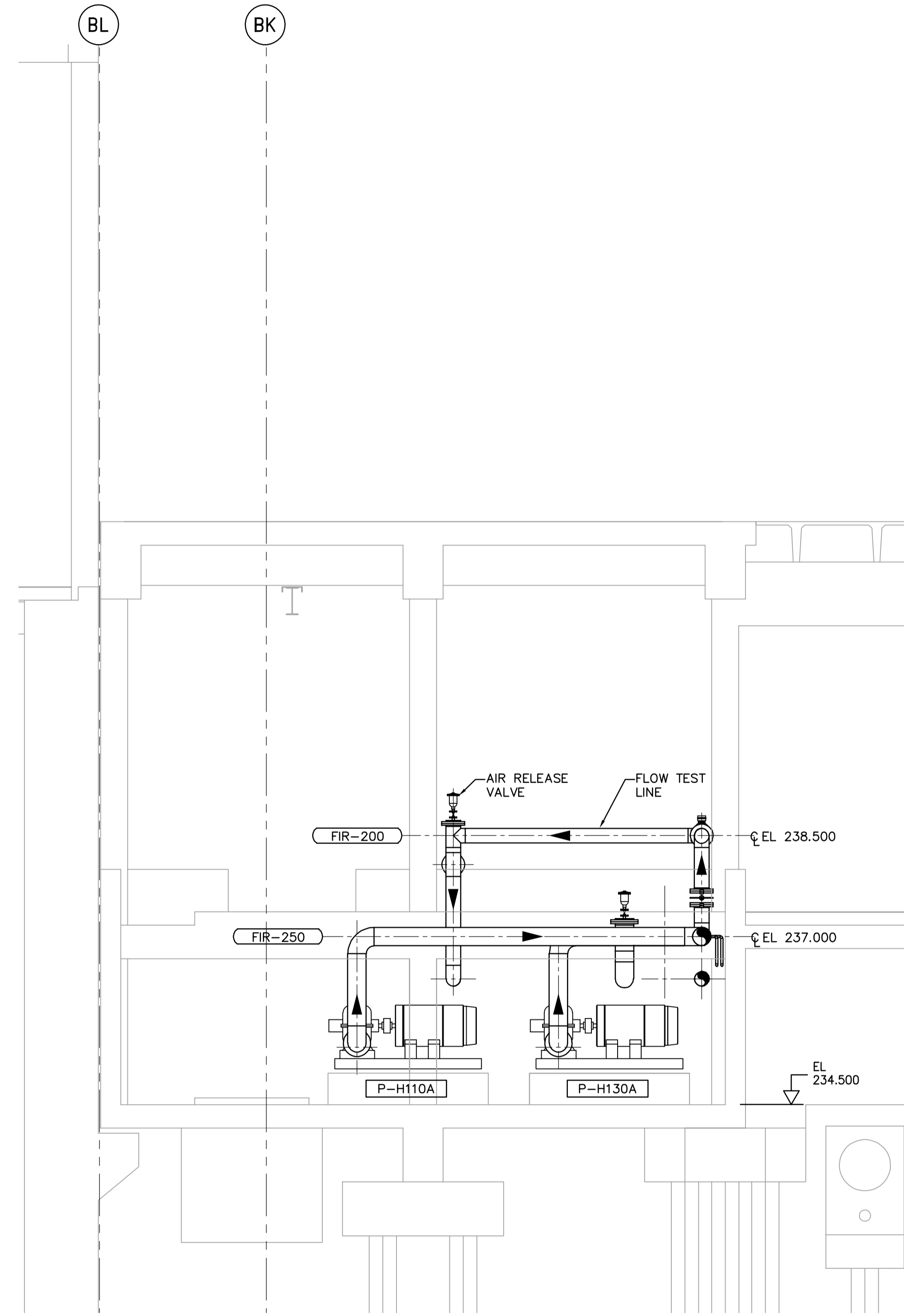
B SECTION WM-H0113 1:50
