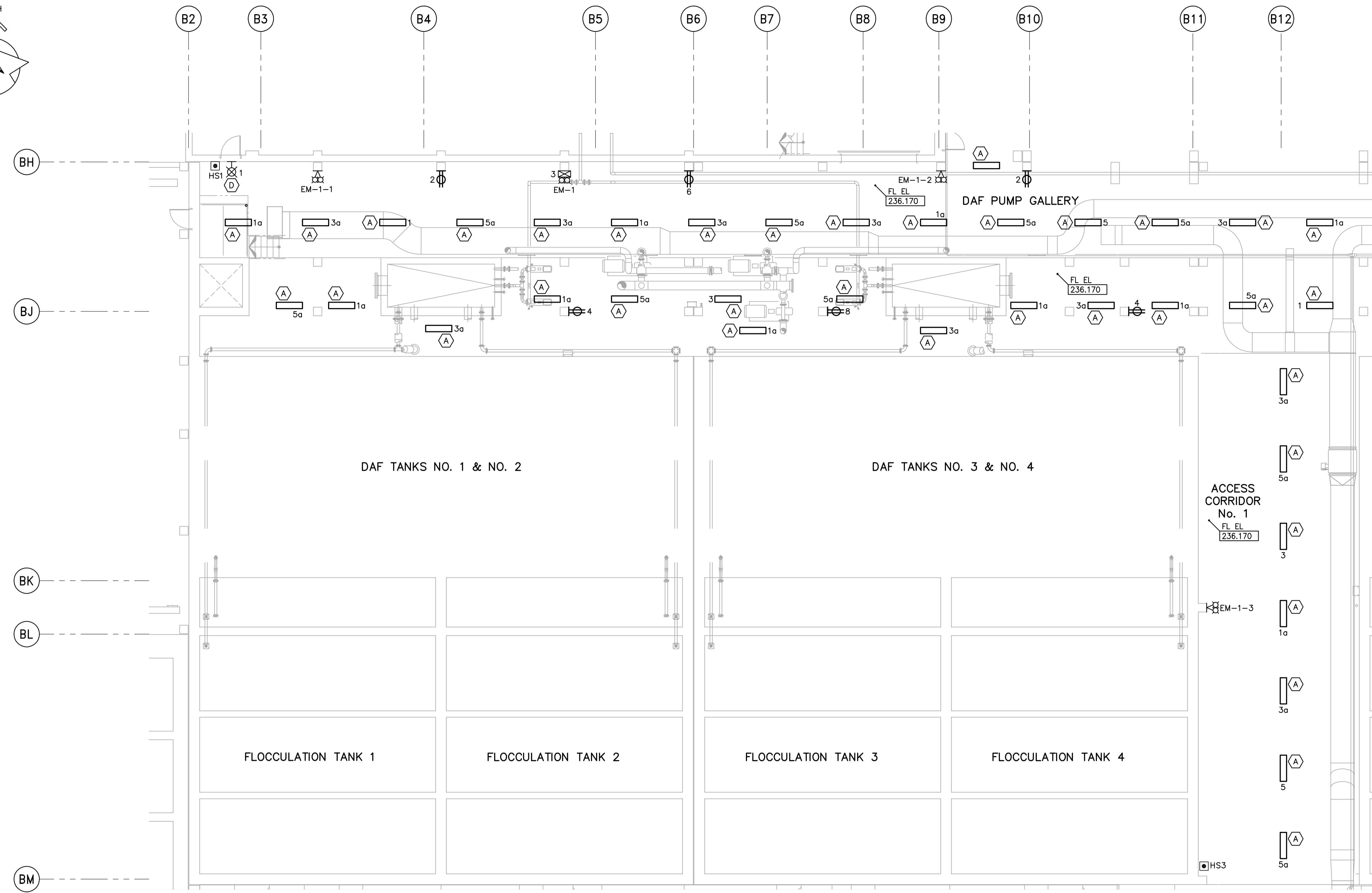
FIRST FLOOR POWER AND LIGHTING PLAN (AREA 1) 1:100
