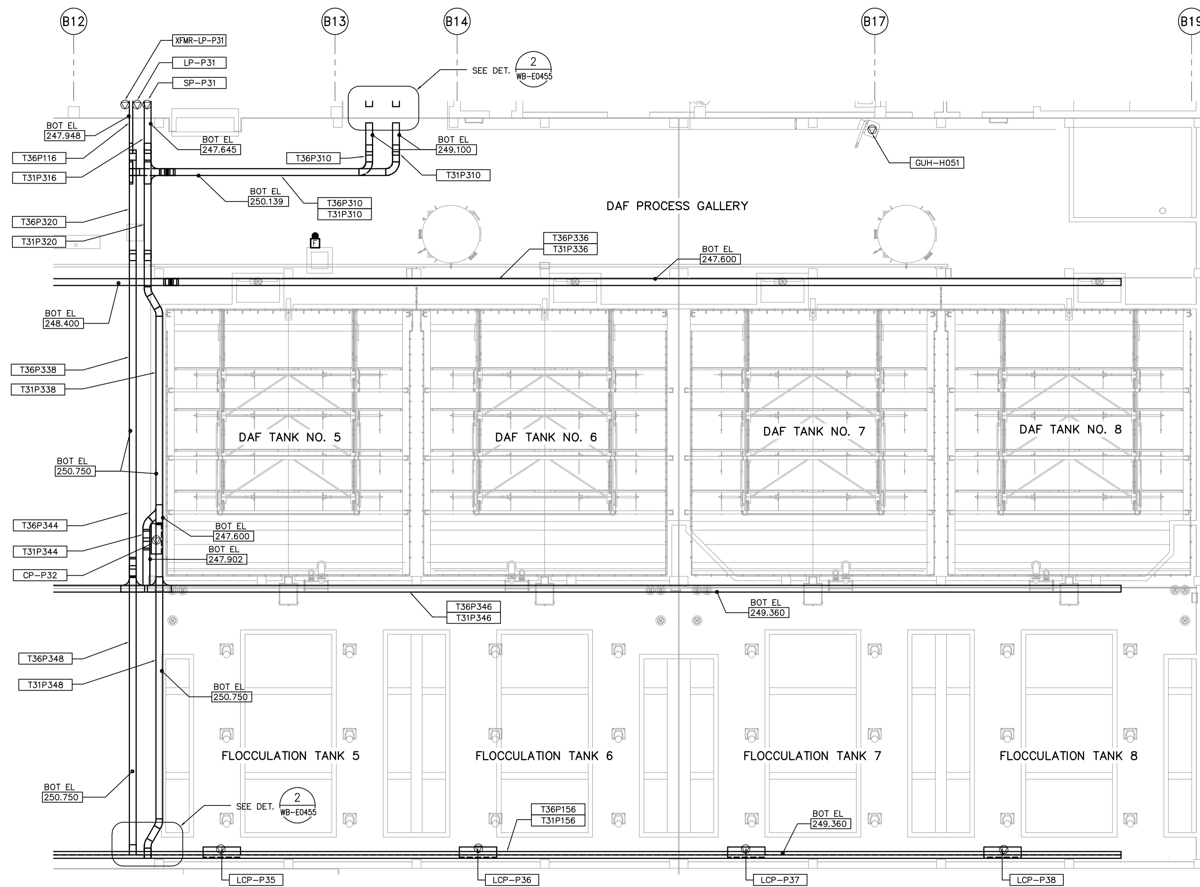
THIRD FLOOR FACILITY PLAN 2 1:100
