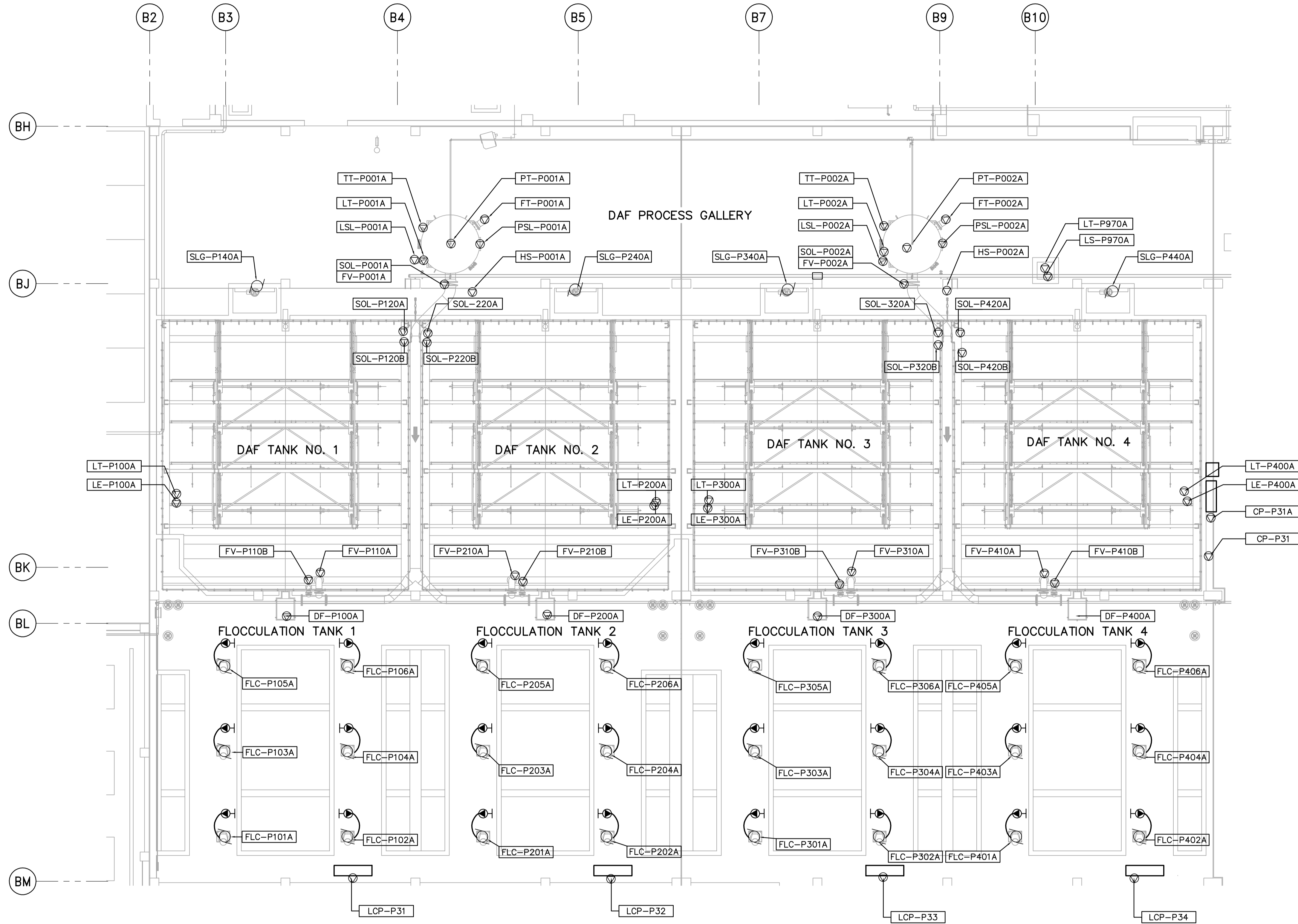
THIRD FLOOR PROCESS PLAN (AREA 1) 1:100
