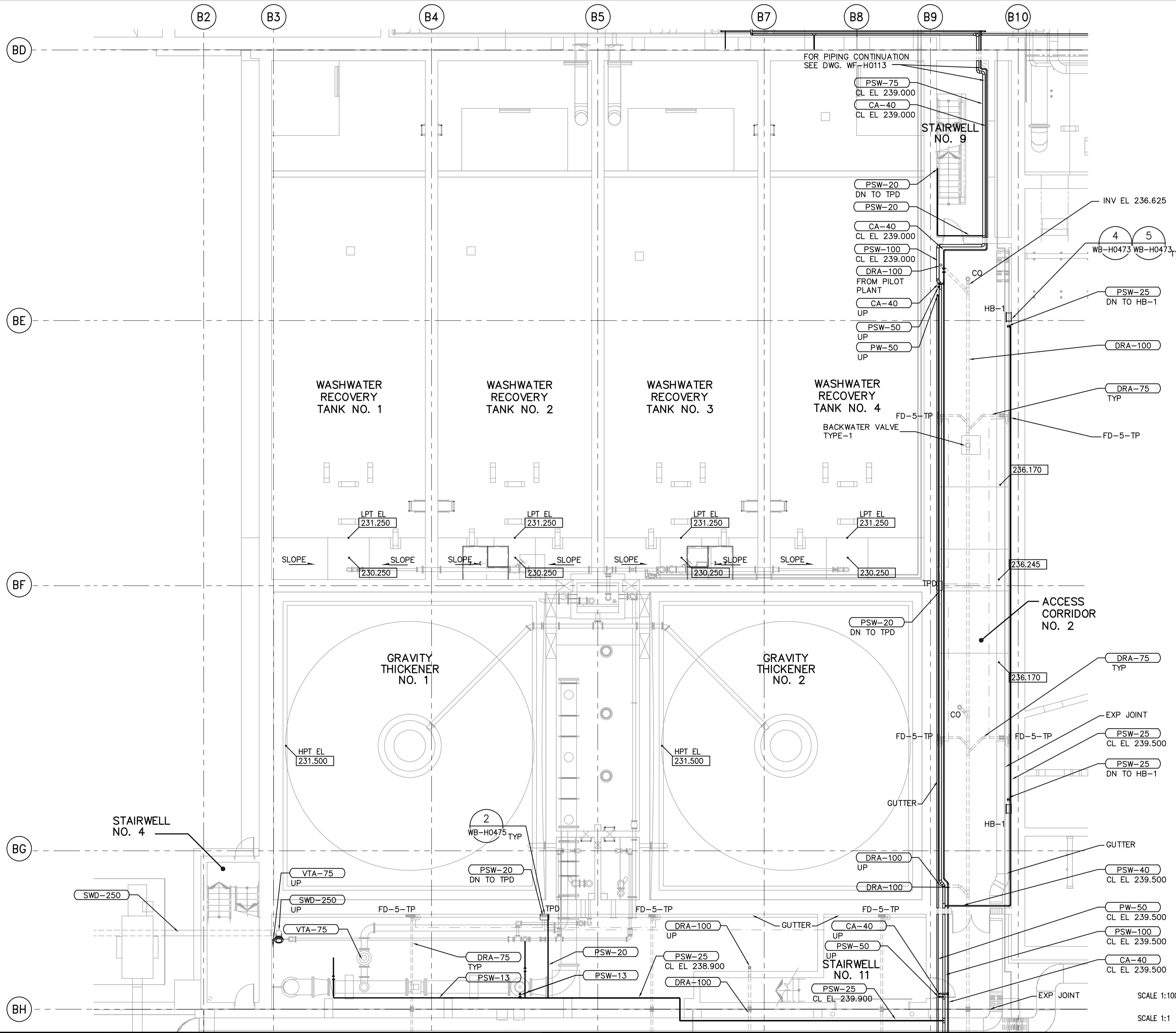
FIRST FLOOR PLAN 1:100
