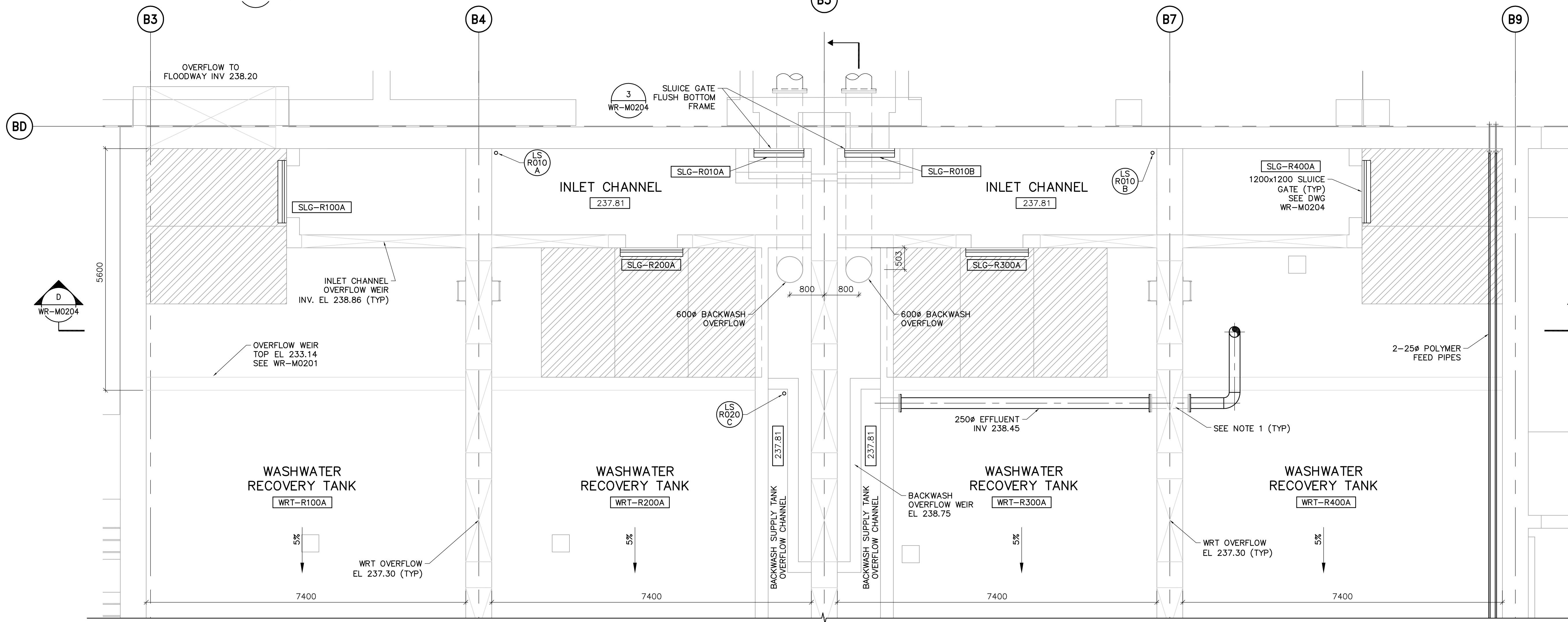
PLAN AT ELEVATION 239.410 WR-M0121 1:50
