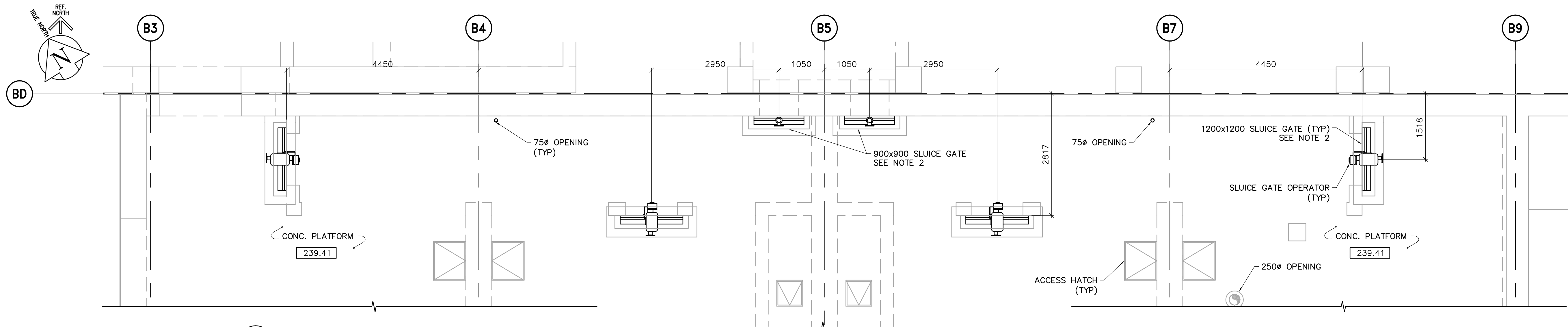
PLAN AT ELEVATION 239.410 WR-M0121 1:50
