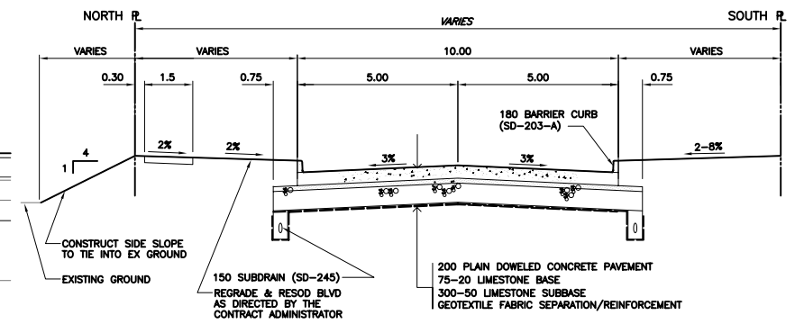
A LUCAS AVENUE CROSS SECTION HOR 1:100, VER 1:50
